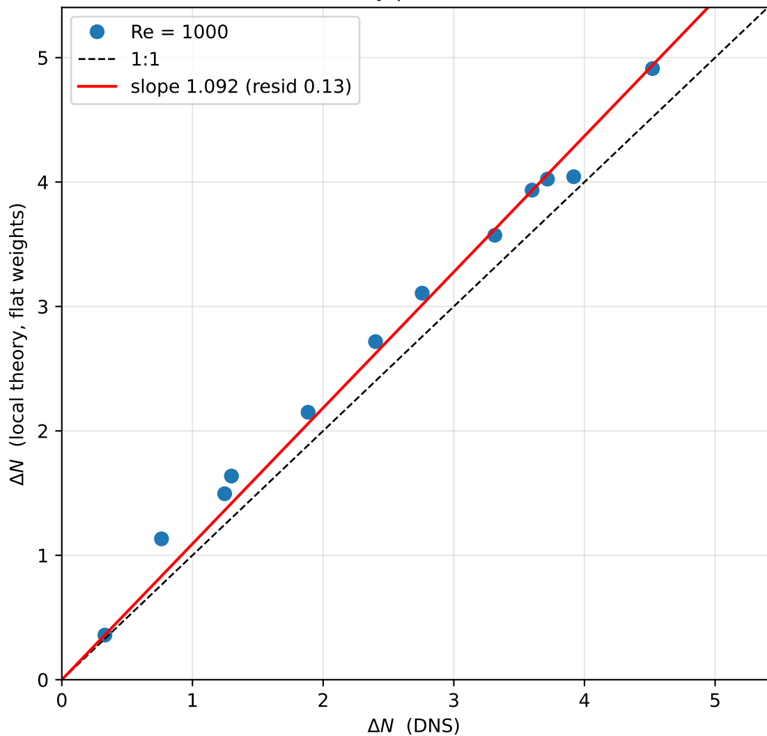
Local stability prediction vs DNS
