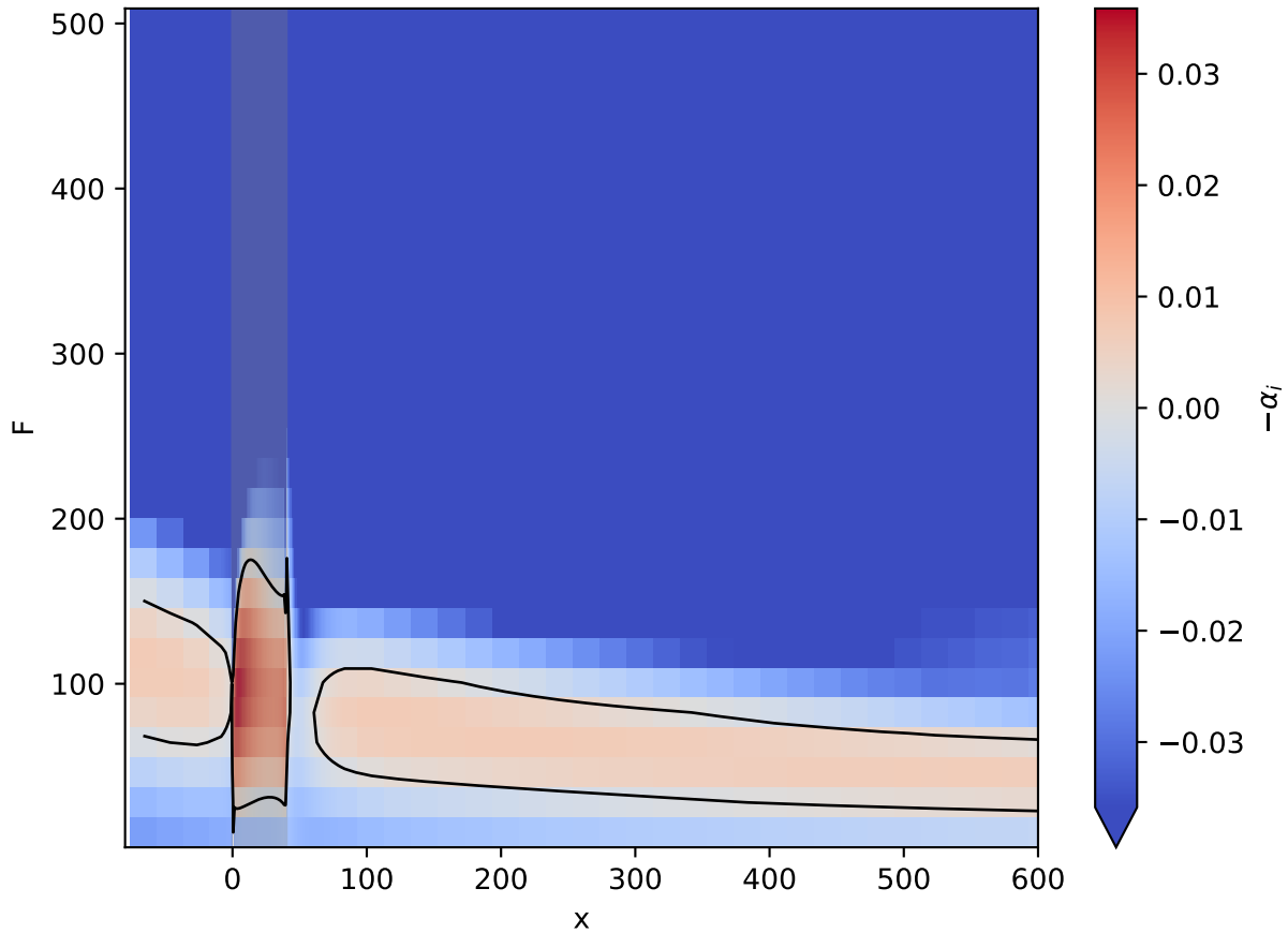
Re1000 d=0.25 w=40: local growth rate
