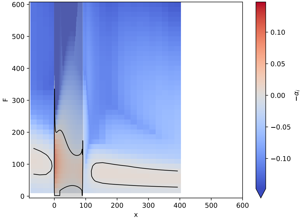
Re1000 d=0.5 w=90: local growth rate
