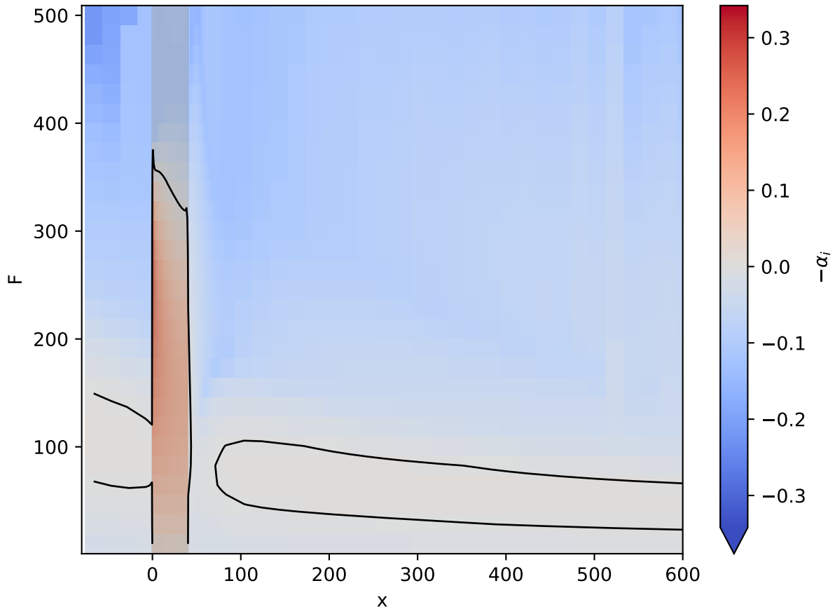
Re1000 d=1.25 w=40: local growth rate
