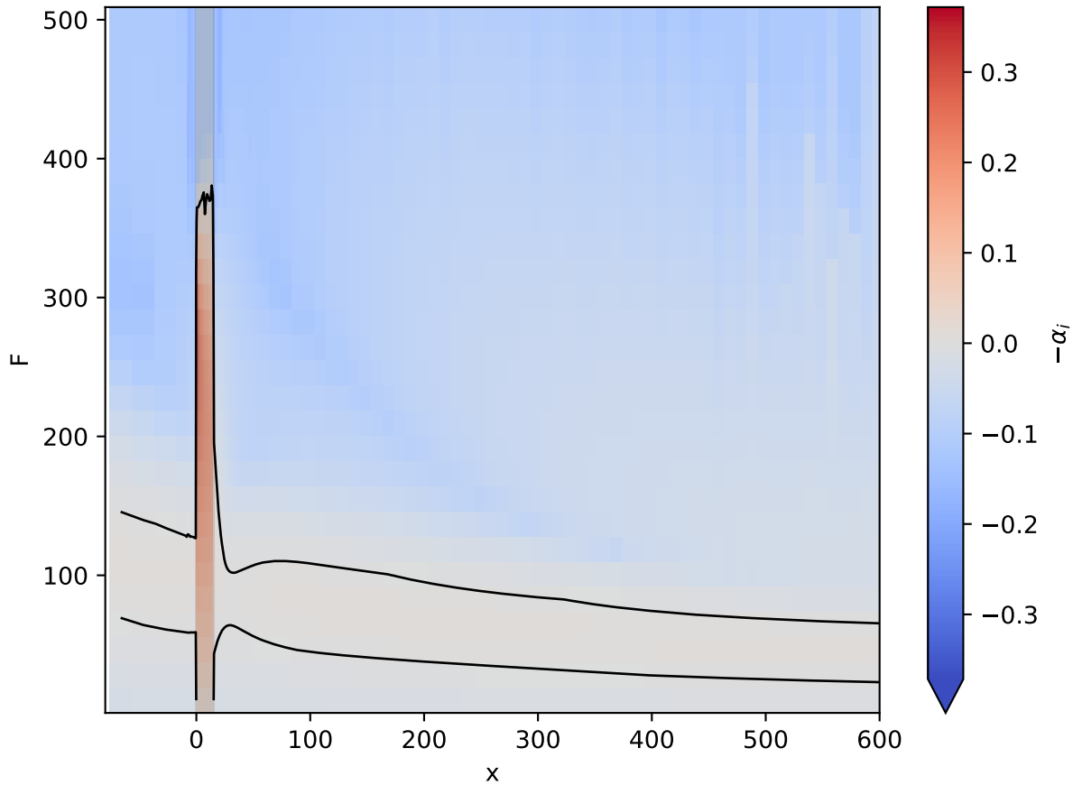
Re1000 d=1.5 w=15: local growth rate
