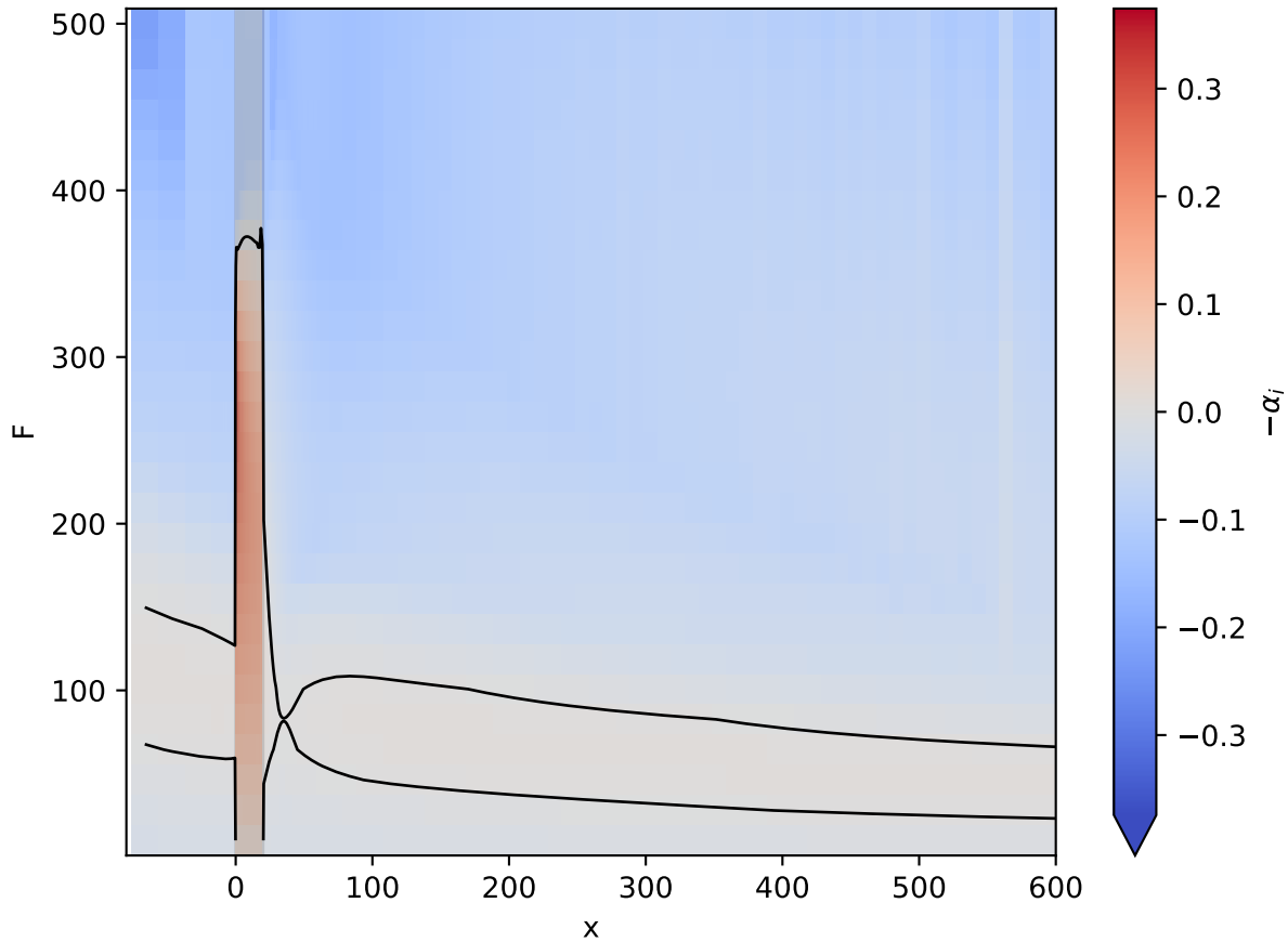
Re1000 d=1.5 w=20: local growth rate
