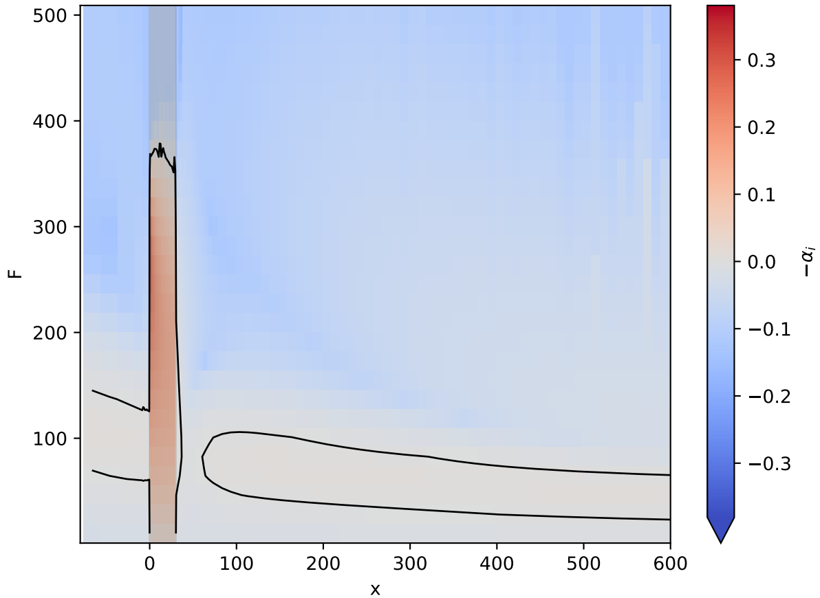
Re1000 d=1.5 w=30: local growth rate
