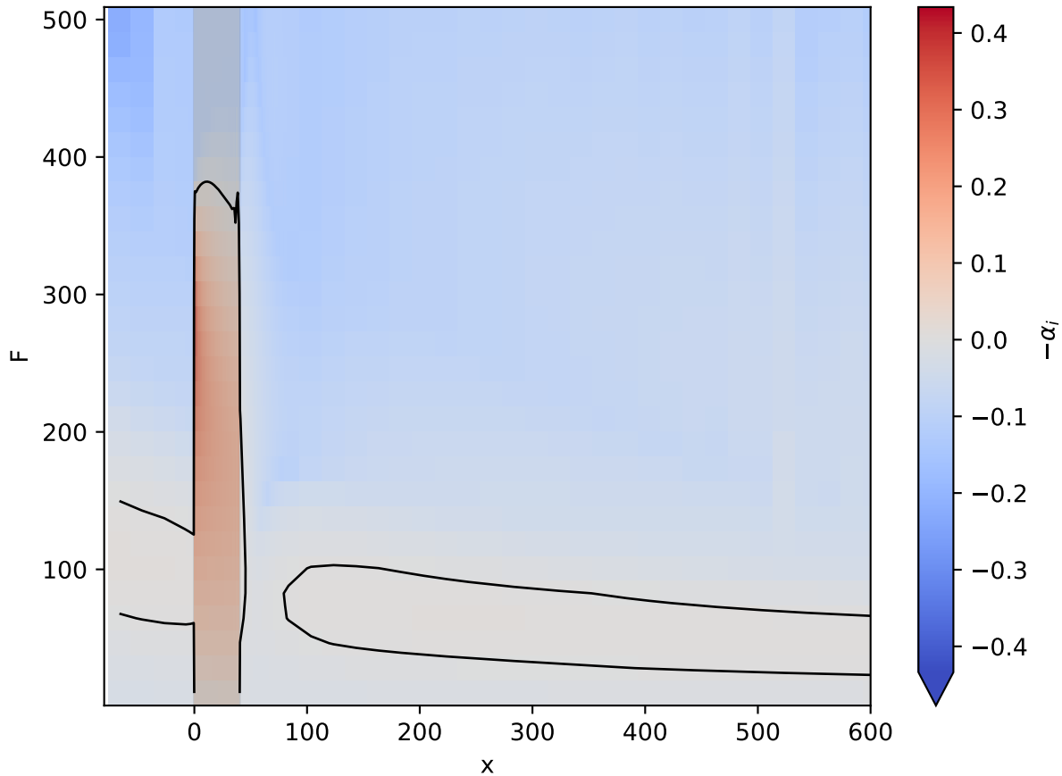
Re1000 d=1.75 w=40: local growth rate
