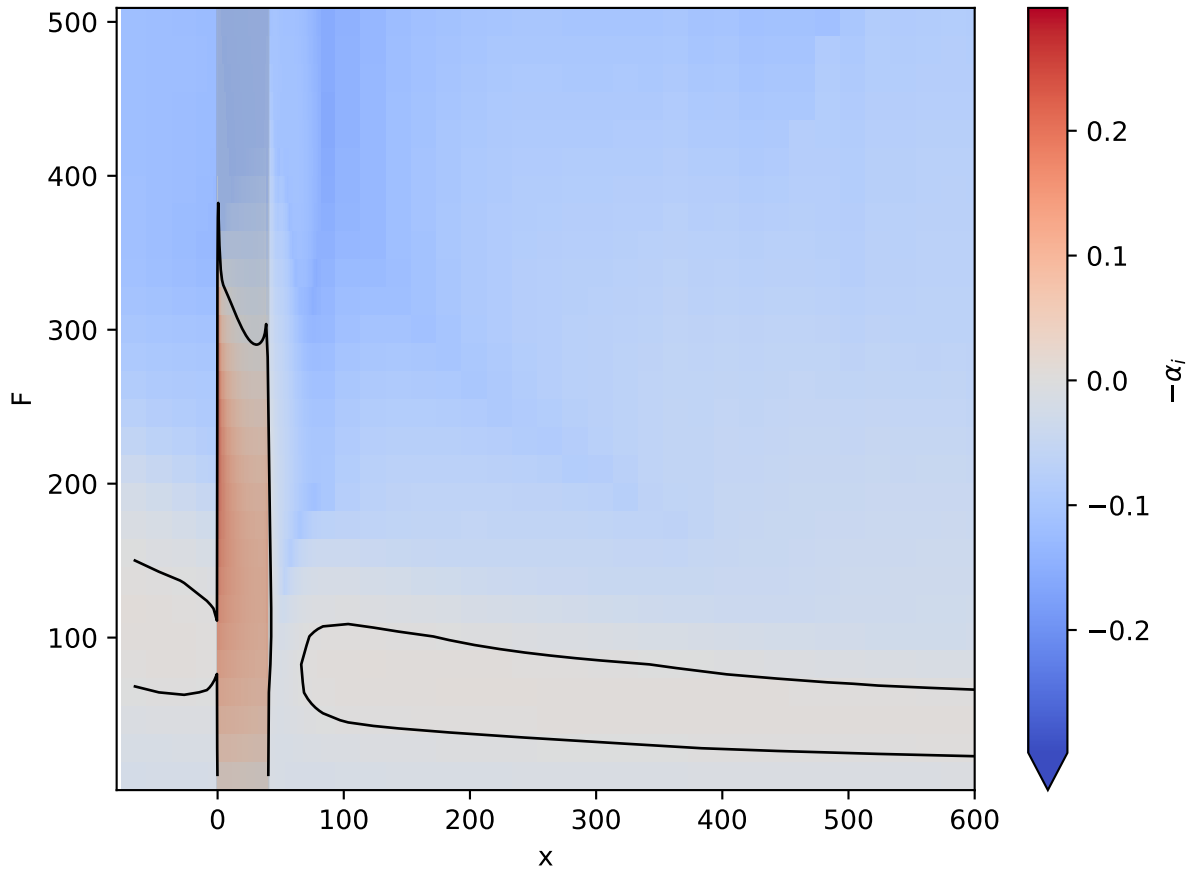
Re1000 d=1 w=40: local growth rate
