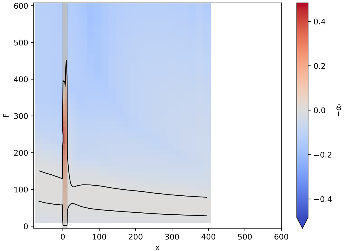
Re1000 d=4 w=12: local growth rate
