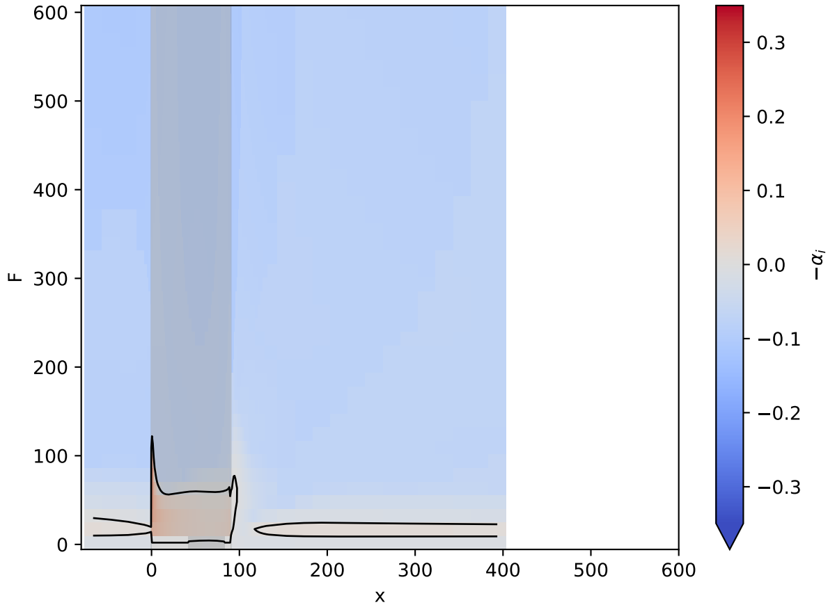
Re3000 d=0.5 w=90: local growth rate
