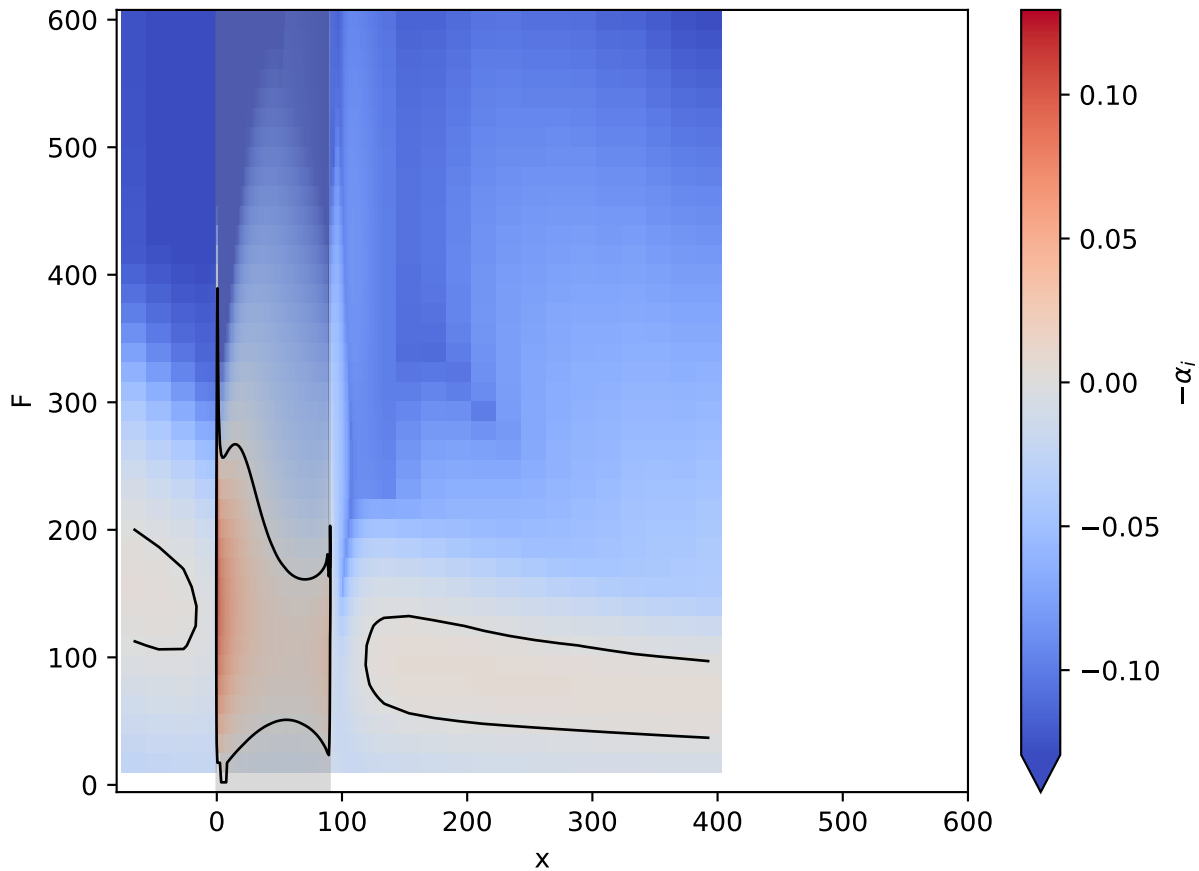
Re800 d=0.5 w=90: local growth rate
