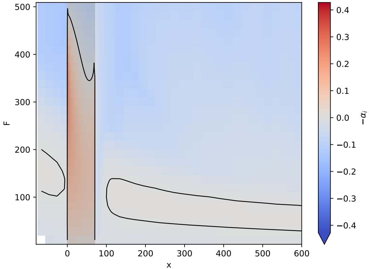
Re800 d=1.5 w=70: local growth rate
