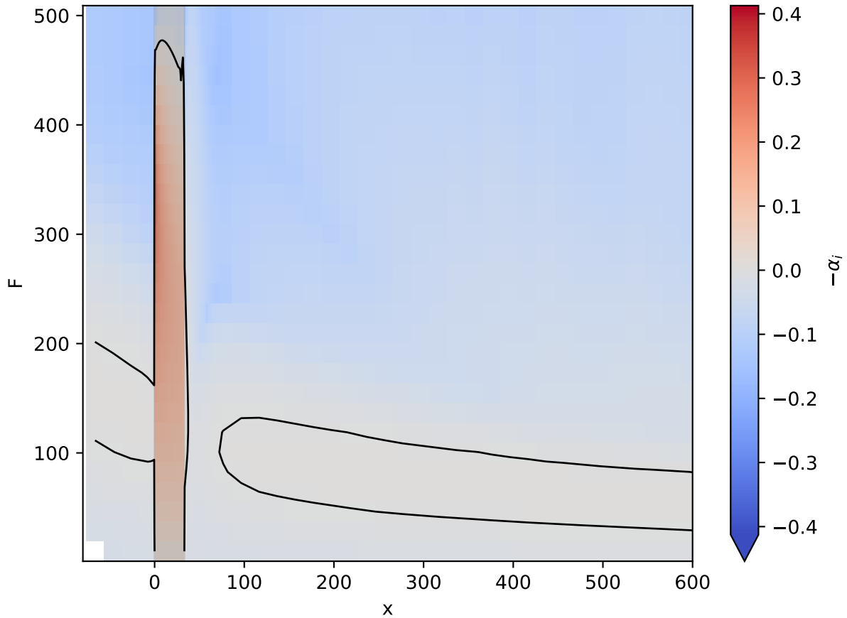
Re800 d=1.75 w=33: local growth rate
