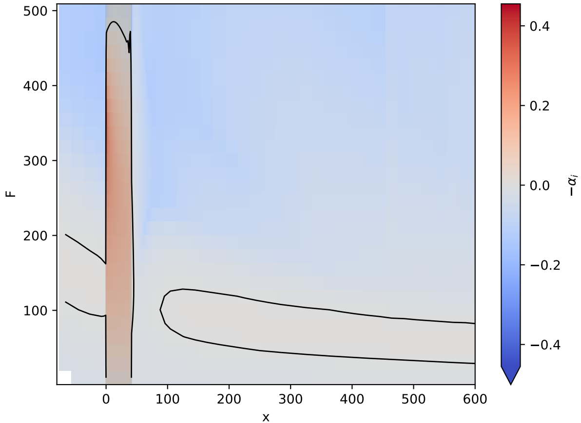
Re800 d=2 w=41: local growth rate
