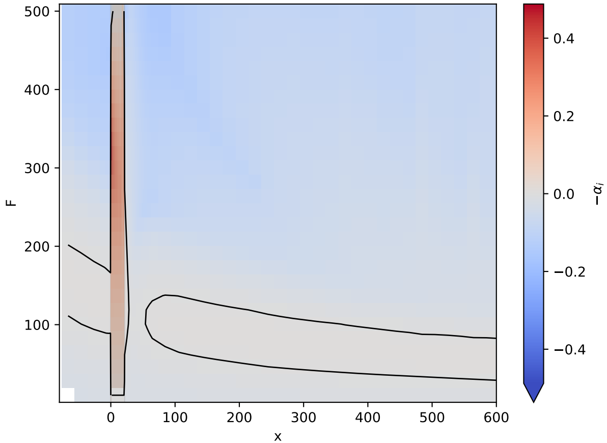
Re800 d=3.5 w=21: local growth rate
