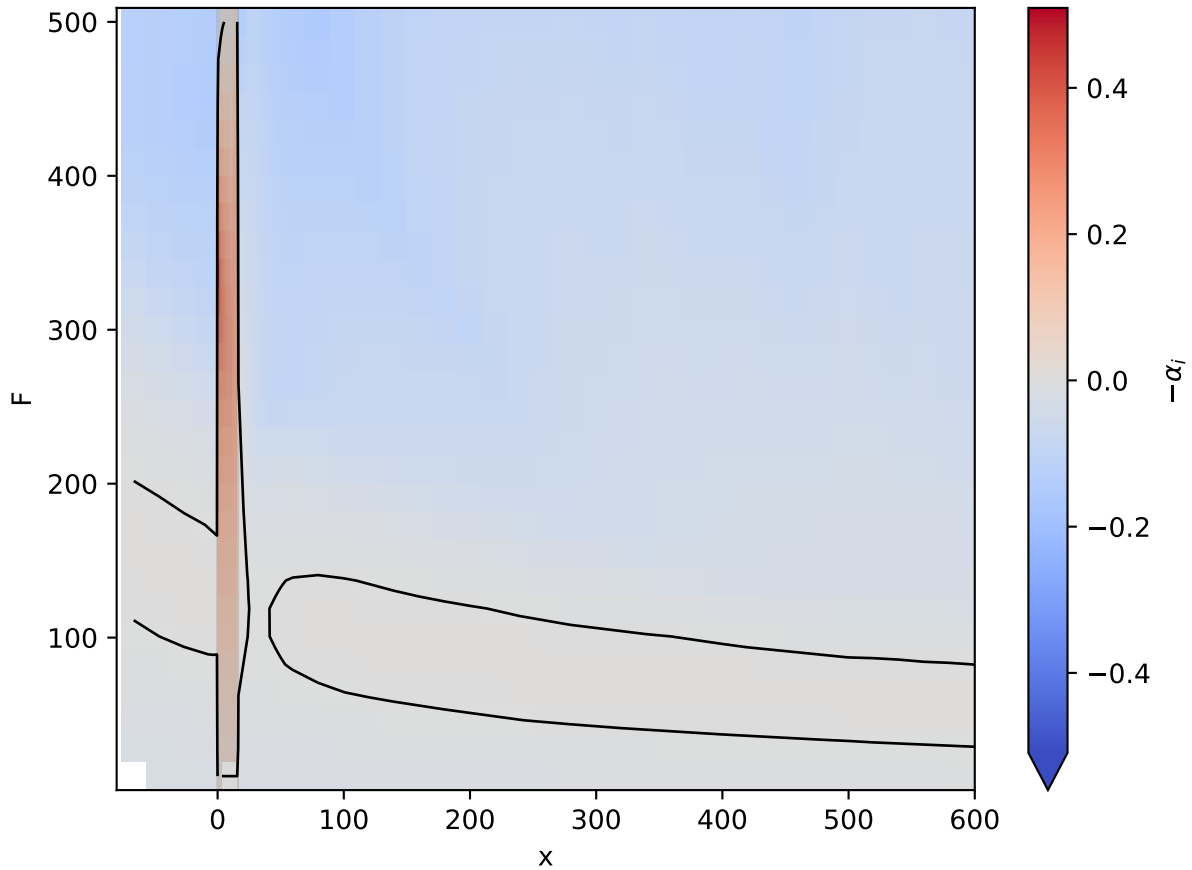
Re800 d=3 w=16: local growth rate
