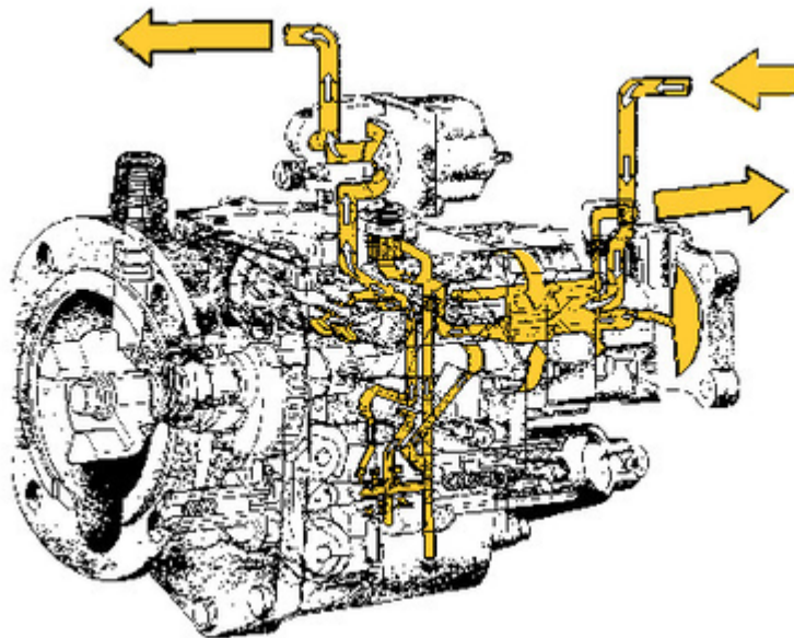
Fuel Flow Through Fuel Pump
