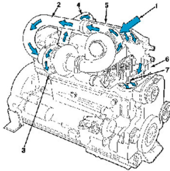
KTTA Intake System
