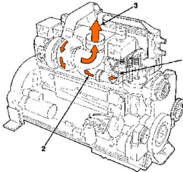
Exhaust System
