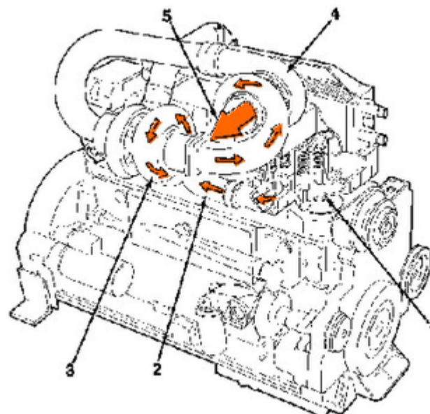
KTTA Exhaust System
