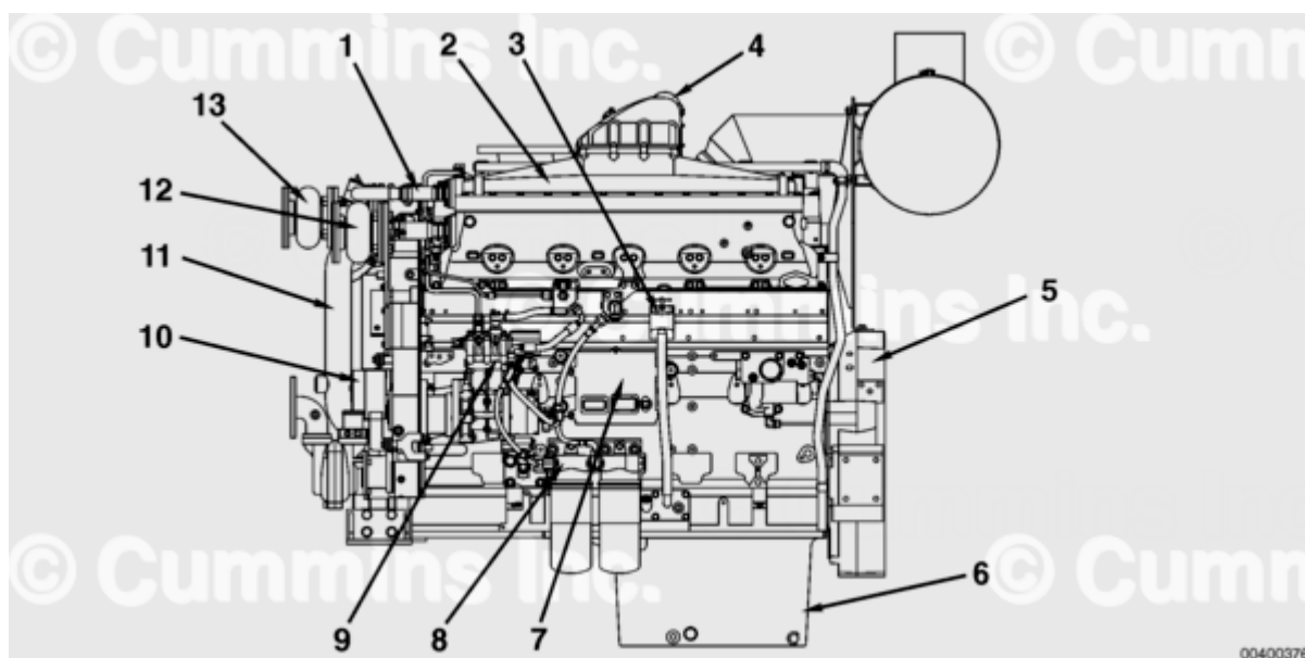
Left View - QSK19 CM850 Keel Cooled
