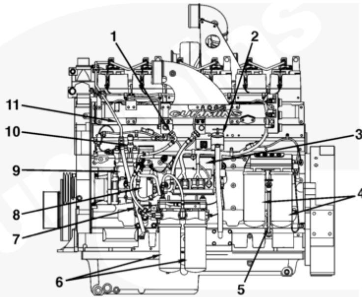
Left View - QSK19 Industrial
