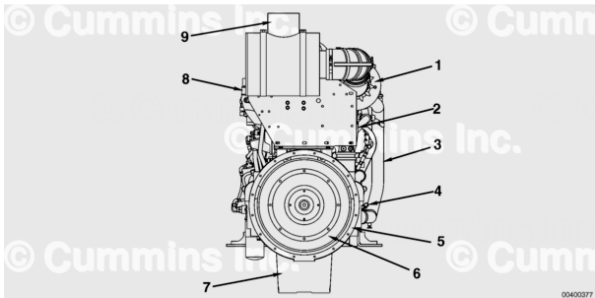
Rear View - QSK19 CM850 Keel Cooled
