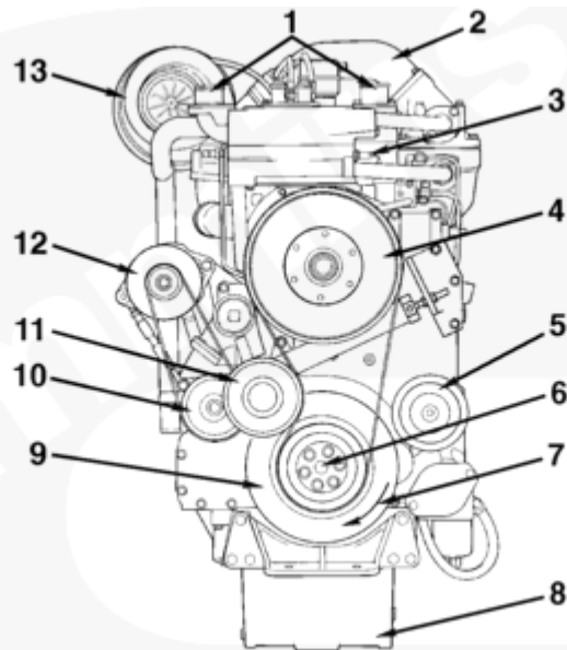
Front View - QSK19
