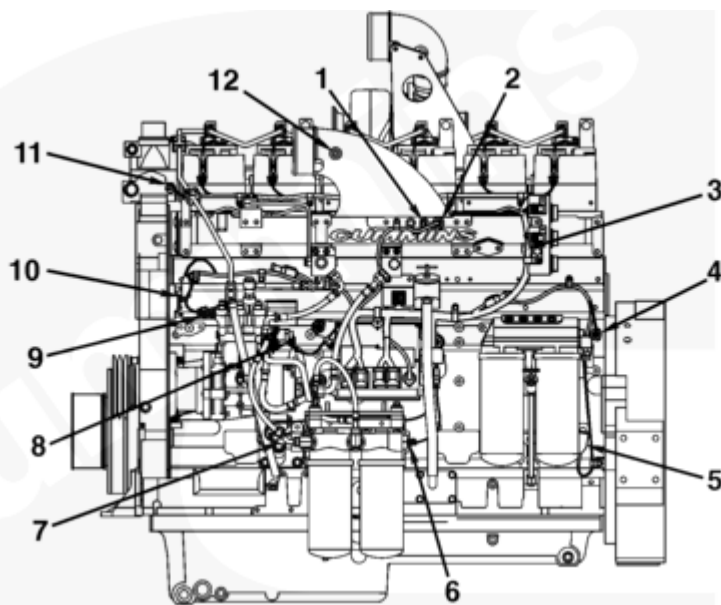
Left View - QSK19 Industrial (Sensor Locations)
