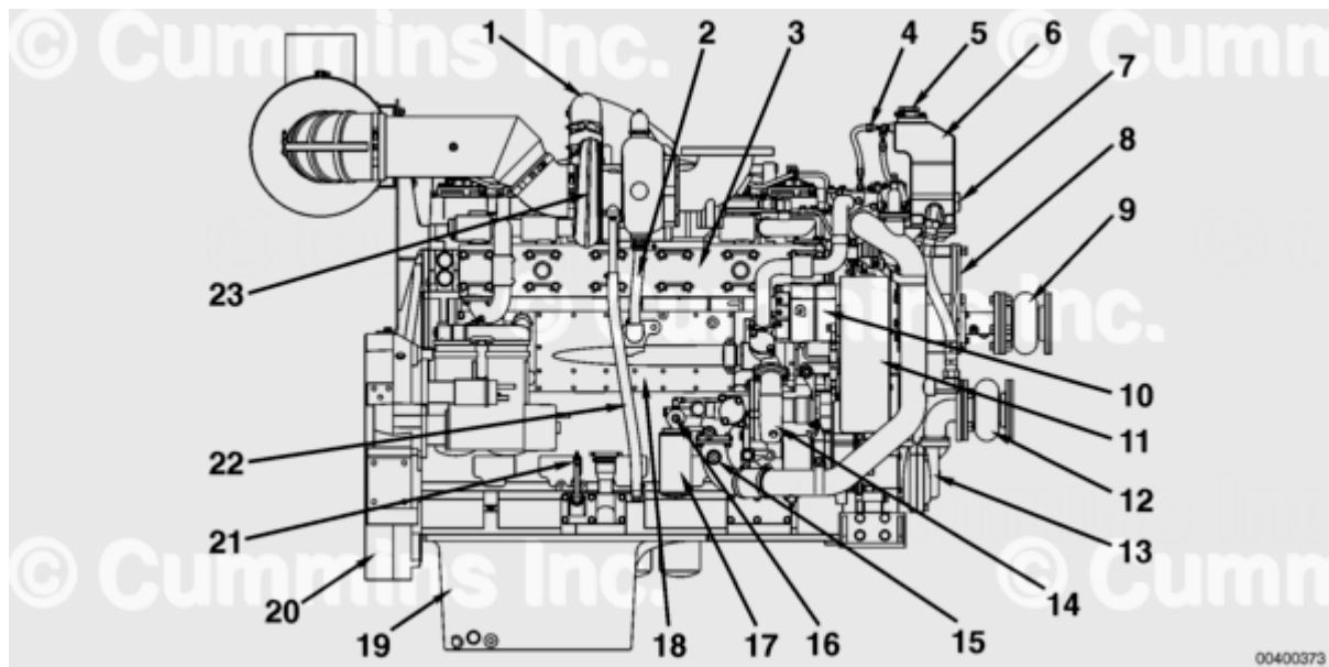
Right View - QSK19 CM850 Heat Exchanger
