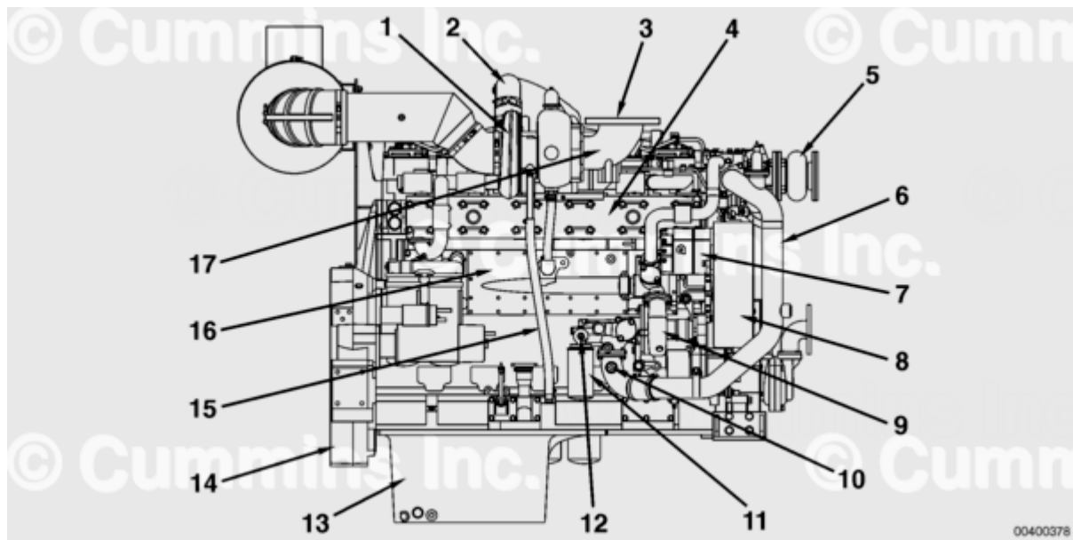
Right View - QSK19 CM850 Keel Cooled
