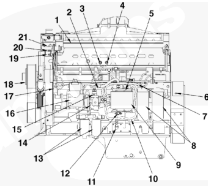
Left View - QSK19
