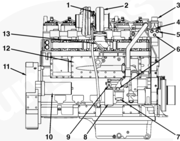
Right View - QSK19 Industrial
