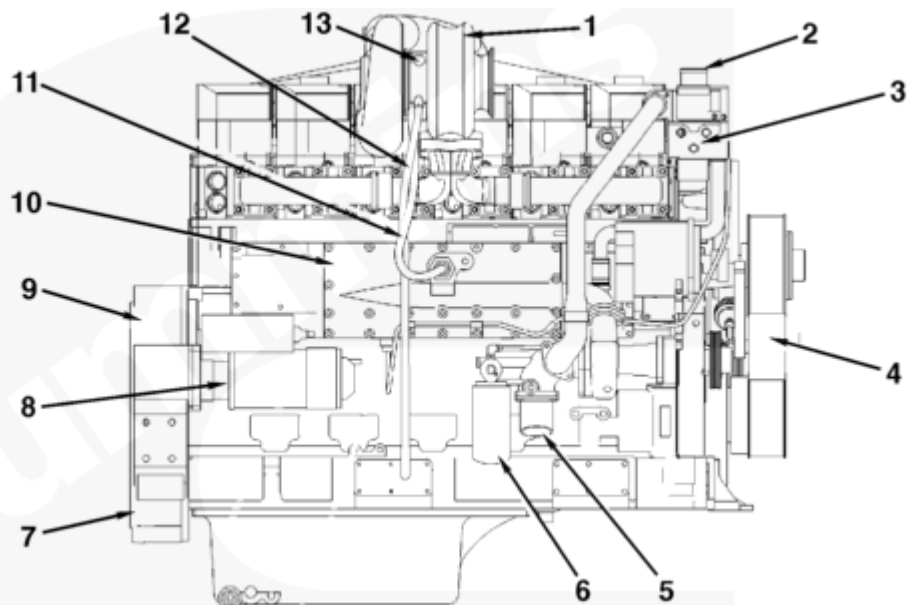
Right View - QSK19
