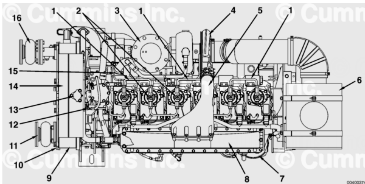
Top View - QSK19 CM850 Heat Exchanger
