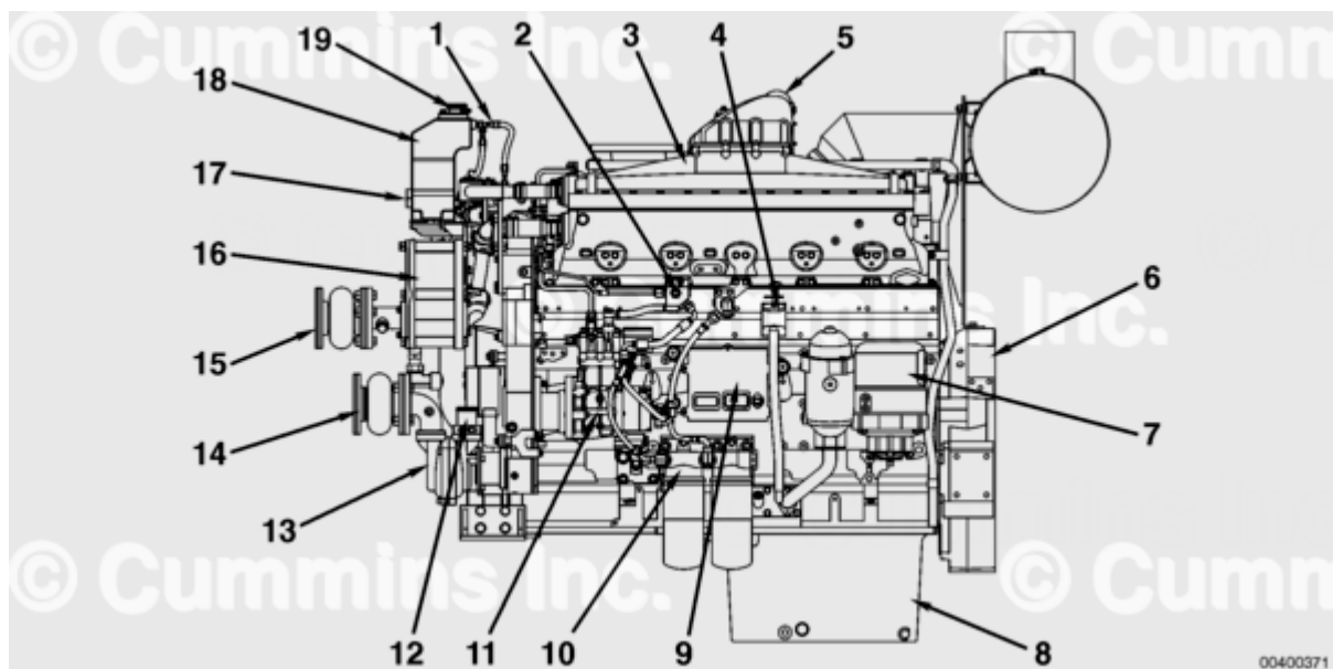
Left View - QSK19 CM850 Heat Exchanger
