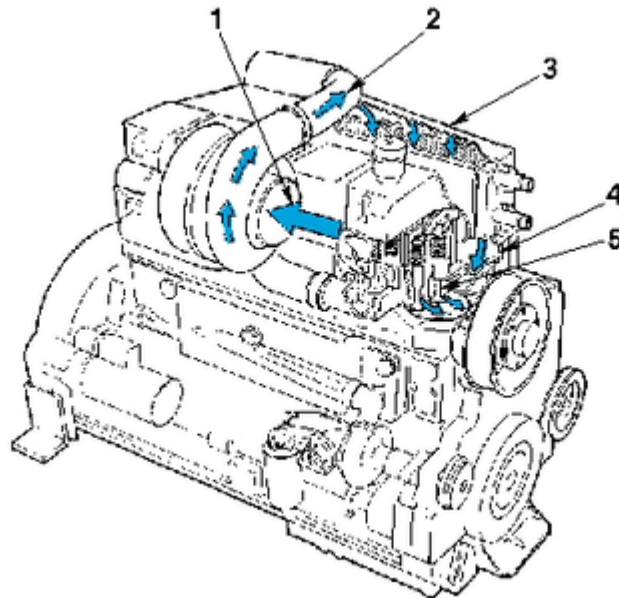
QSK19 Engine - Mechanically Actuated Injector
