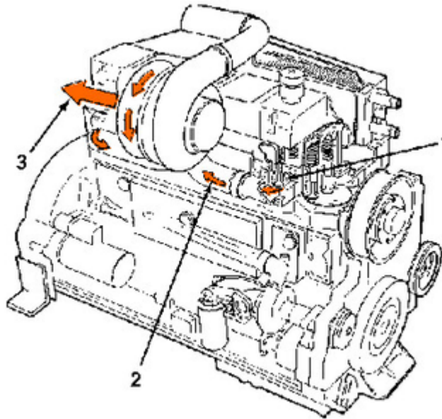
QSK19 - Mechanically Actuated Injector
