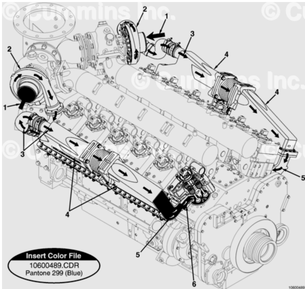
QSK38 Marine Intake Air Flow (QSK50 similar)
