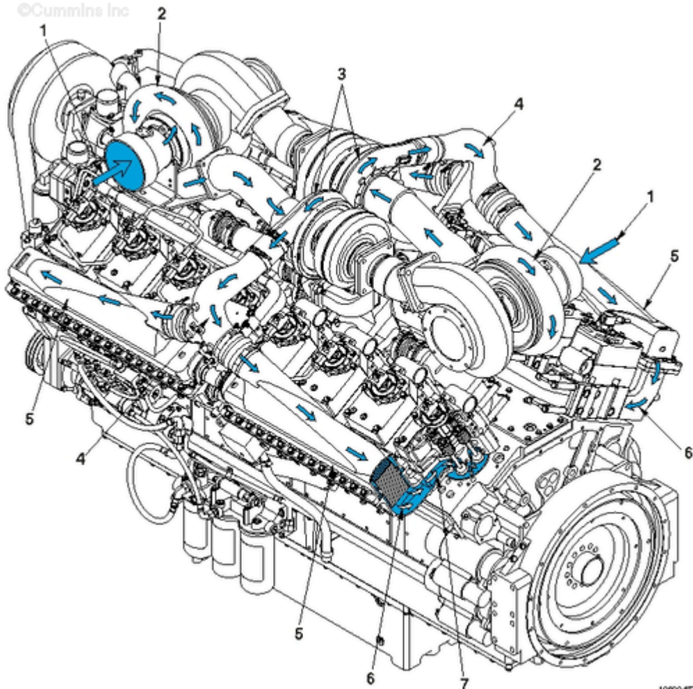
QSK50 Intake Air Flow
