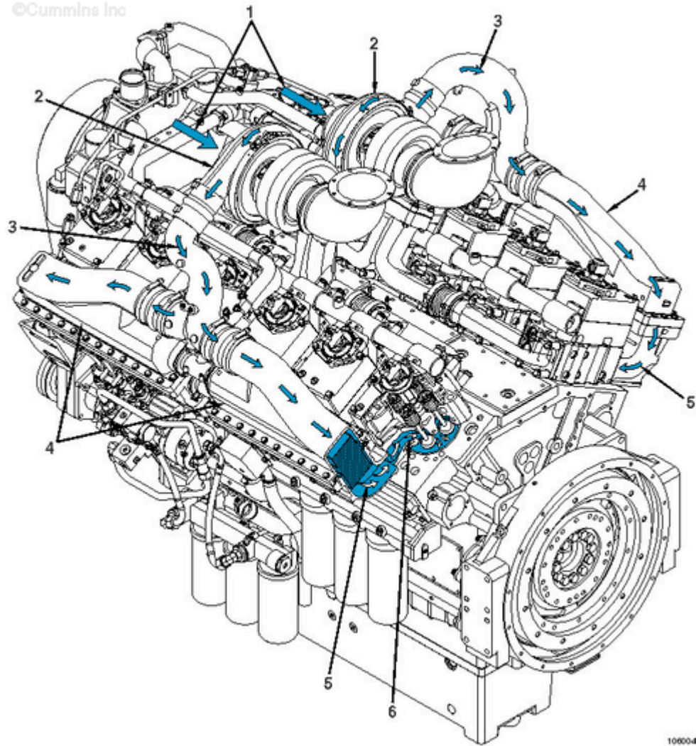
QSK38 Intake Air Flow
