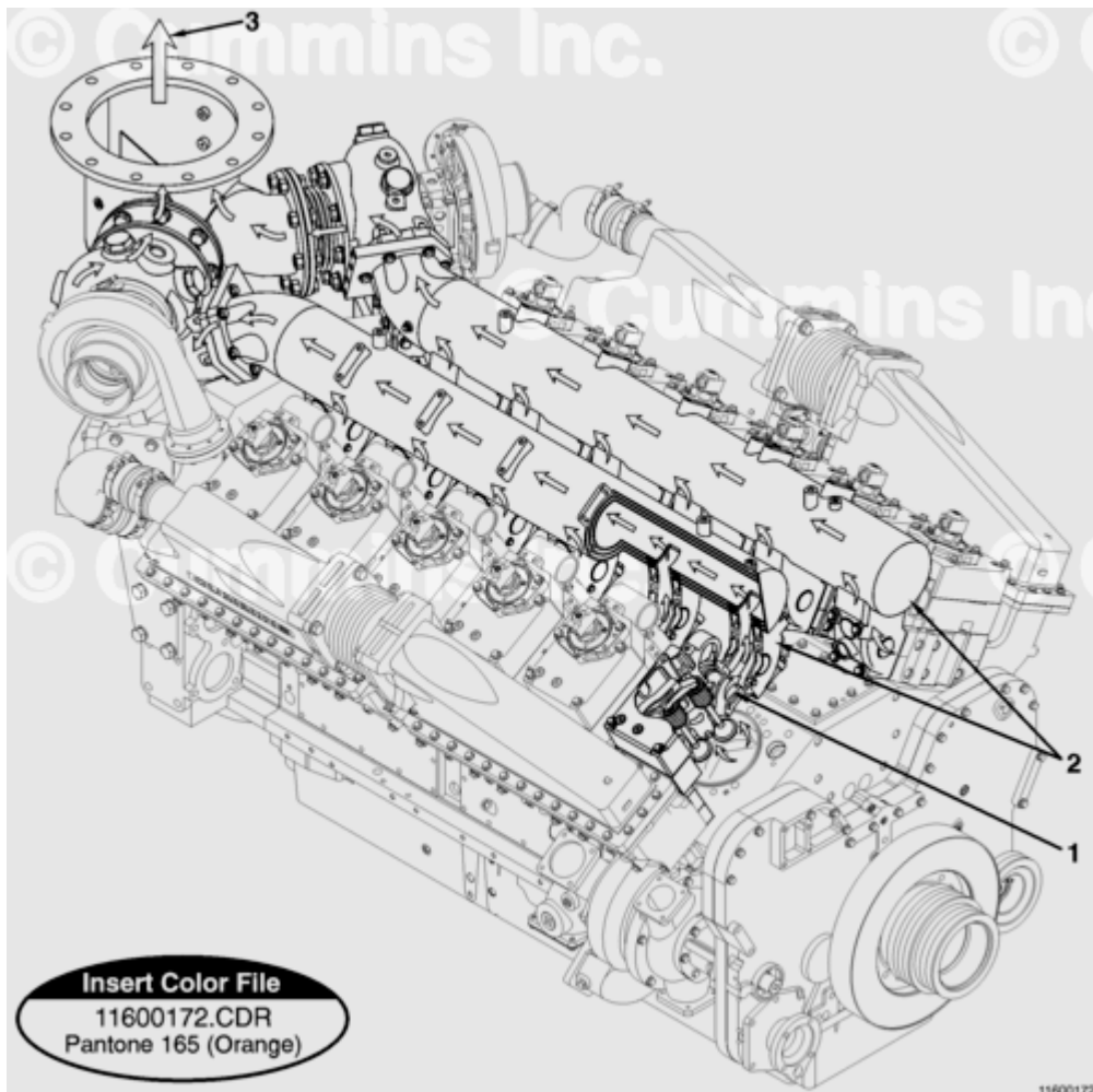
QS38 Marine Exhaust Flow (QS50 Similar)
