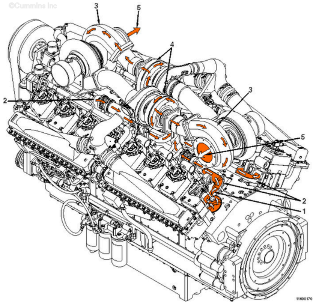
QSK50 Exhaust Flow
