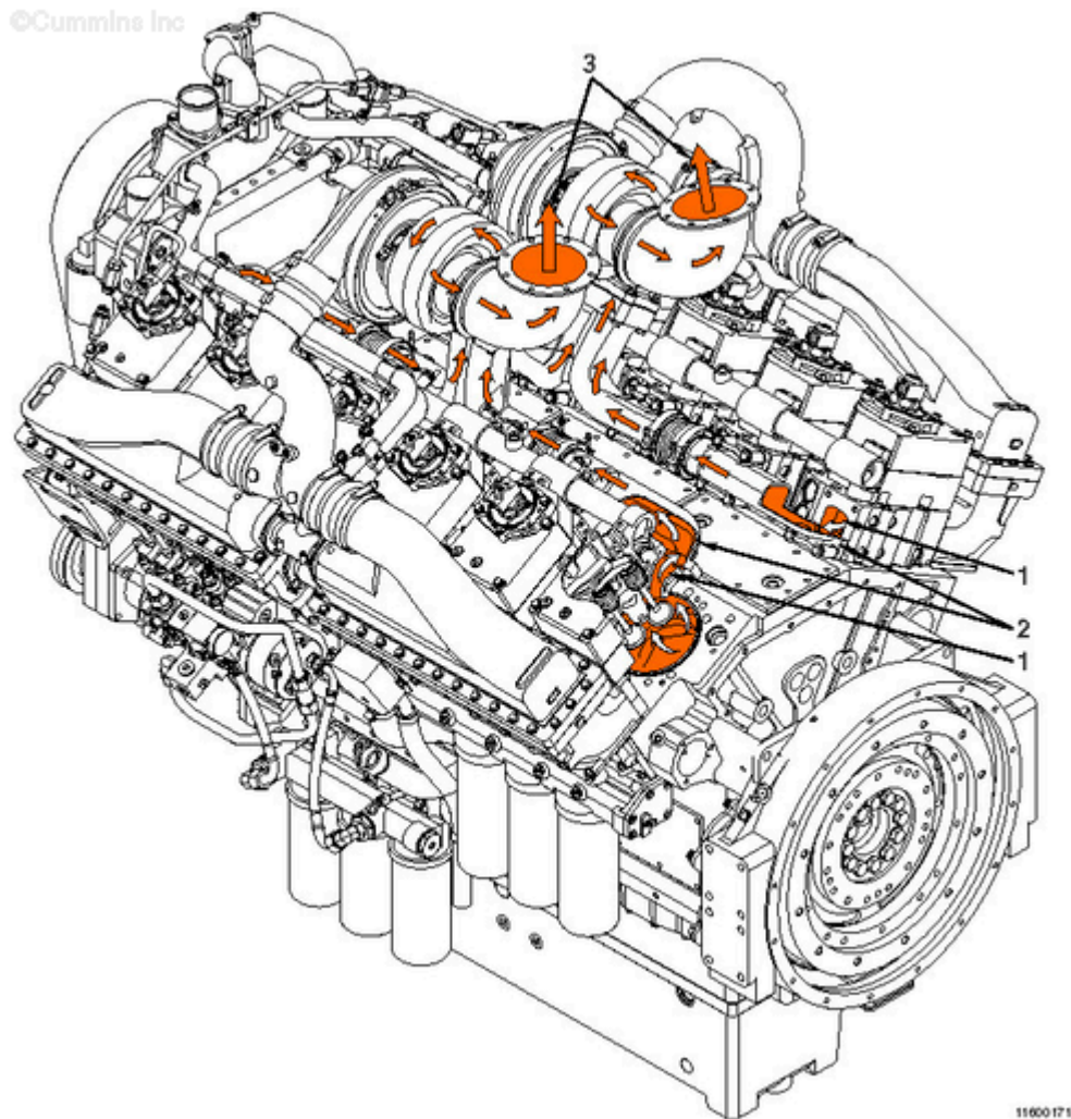
QSK38 Exhaust Flow
