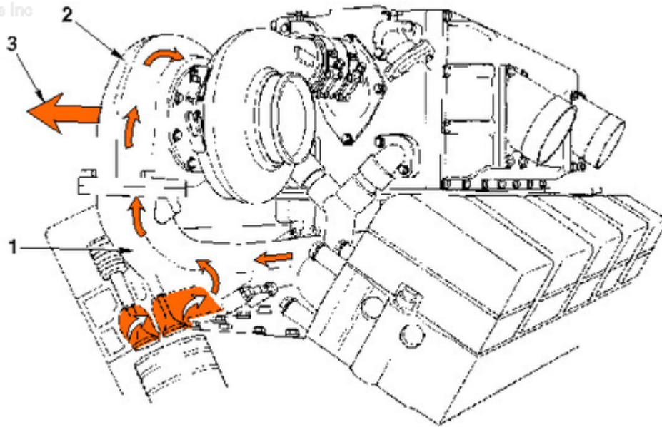
Center Mount Aftercooler
