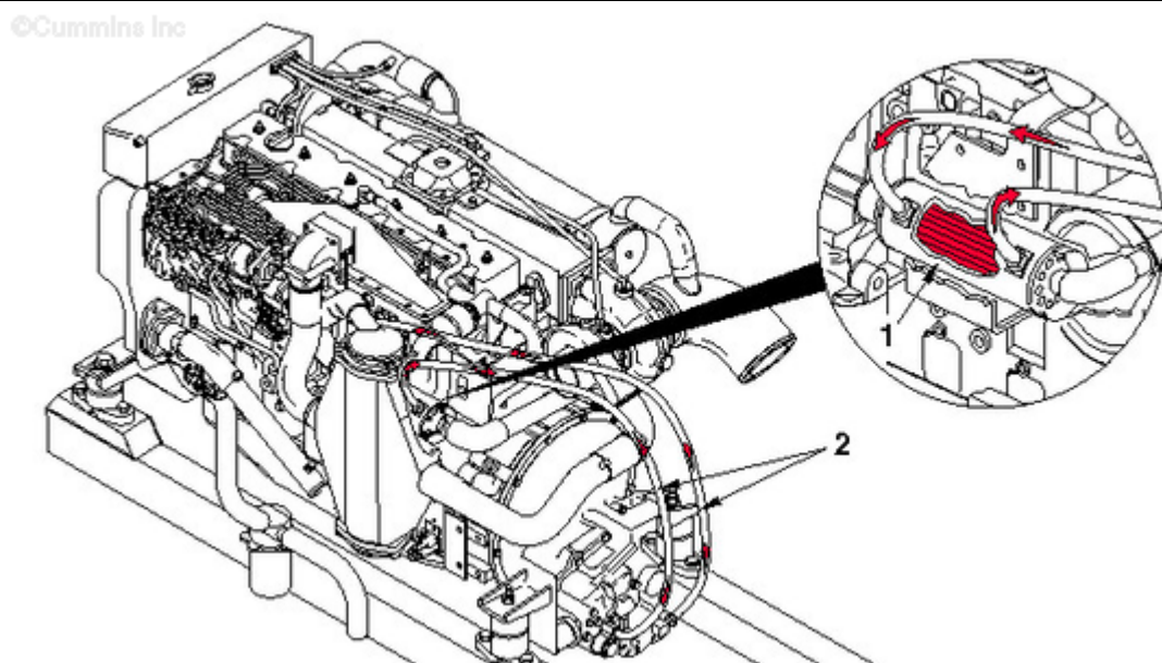
Sea Water Aftercooled
