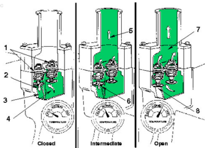
Thermostat
