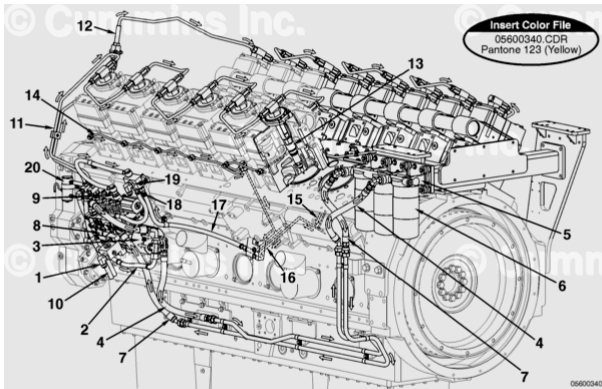
QSK60 Stage 2 Fuel Filtration
