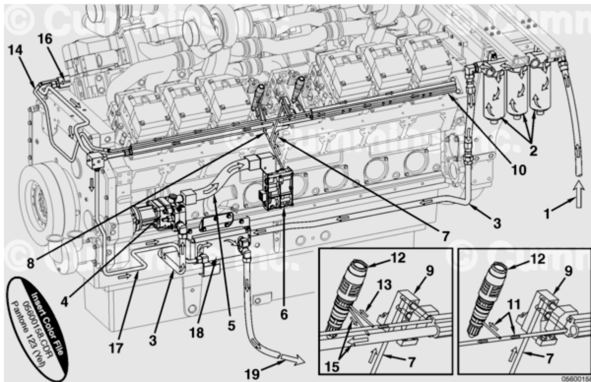
QSK60 Fuel System - Marine with Mechanically Actuated Injector
