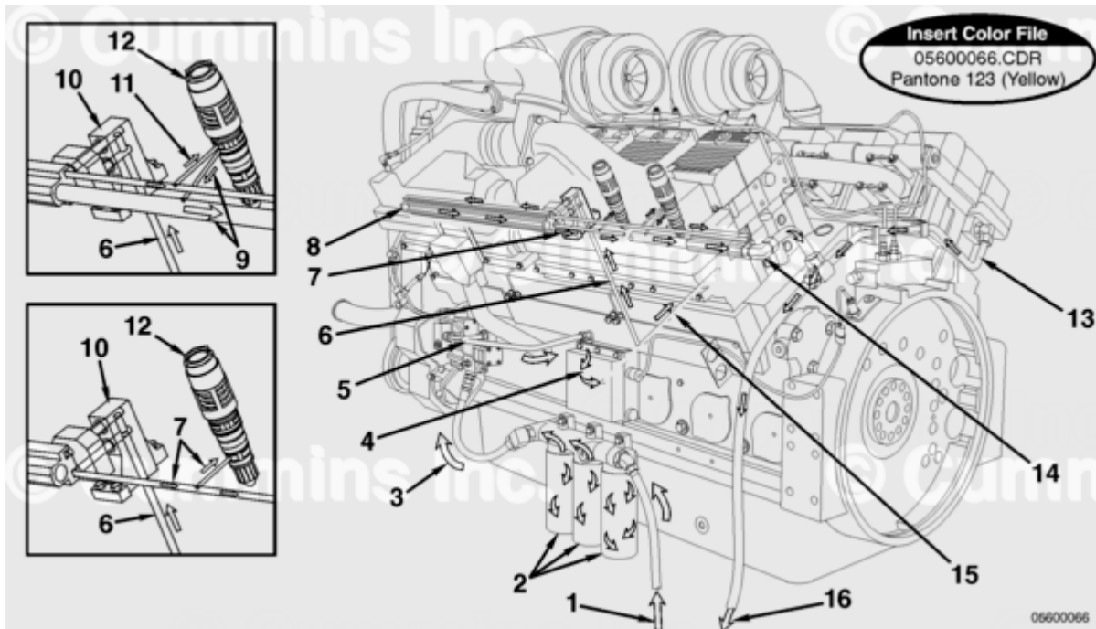
Fuel System - Industrial and Power Generation
