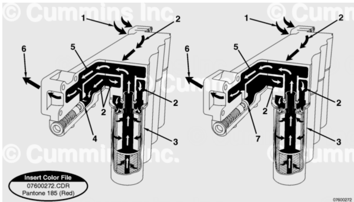
Full-Flow Lubricating Oil Filter Head
