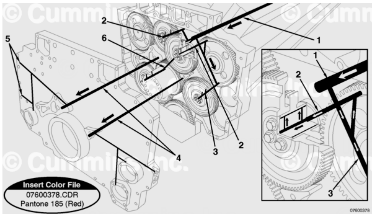
Front Gear Train
