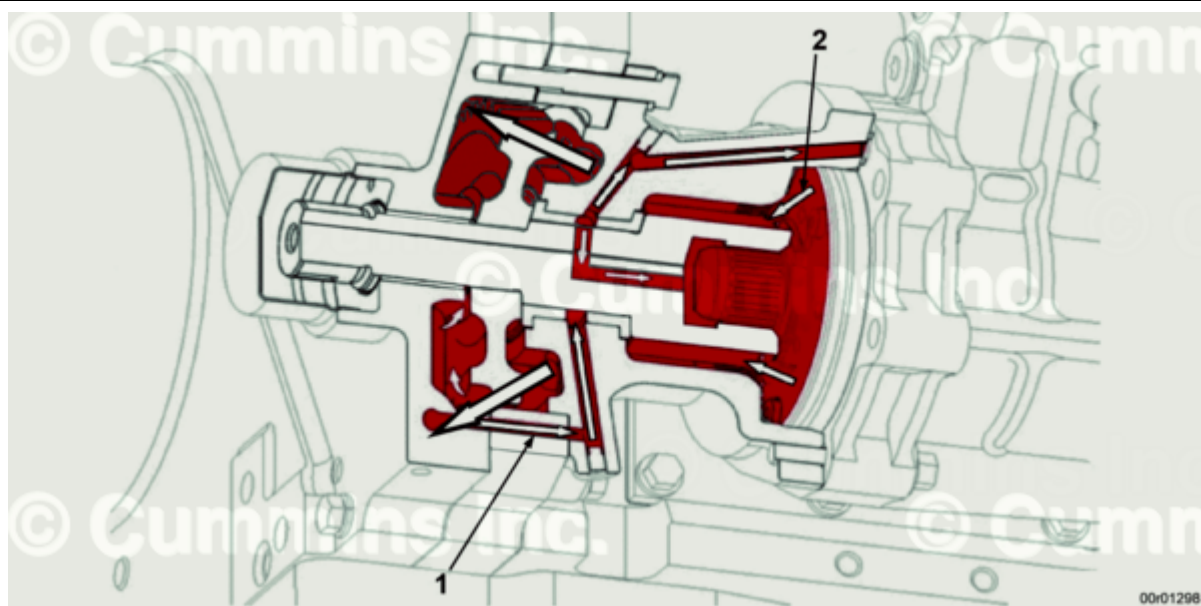
Fuel Pump Lubrication - with Electronically Actuated Injectors
