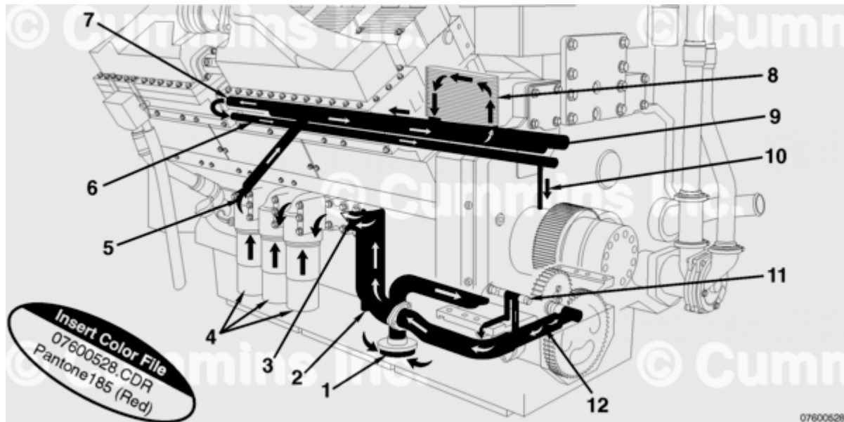
Lubricating Oil System
