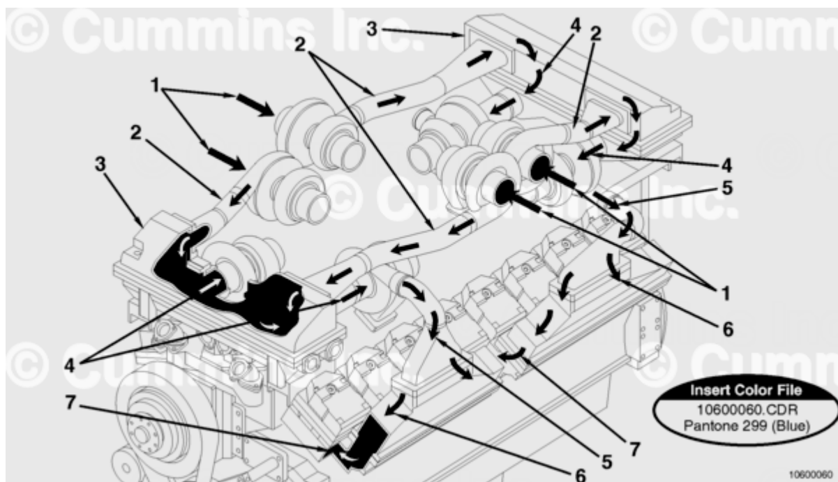
QSK60 Intake System- Two Stage
