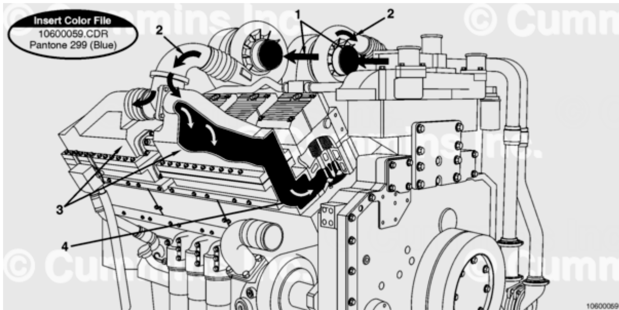
QSK45 Intake System - Single Stage
