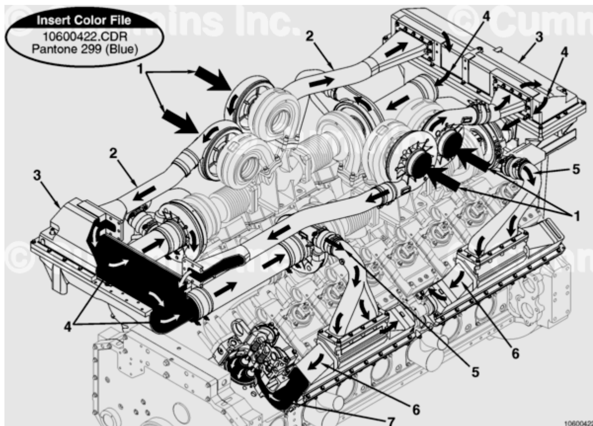
QSK60 Intake System- Two Stage
