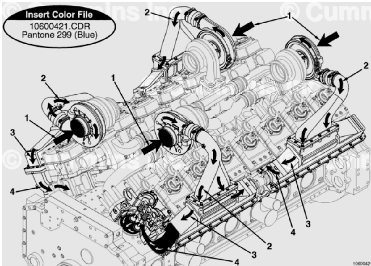
QSK60 Intake System- Single Stage
