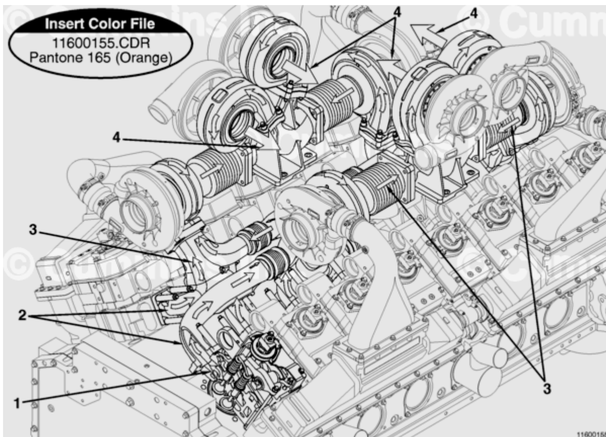
QSK60 Exhaust System - Two-Stage Turbocharger, Aftercooled and Intercooled
