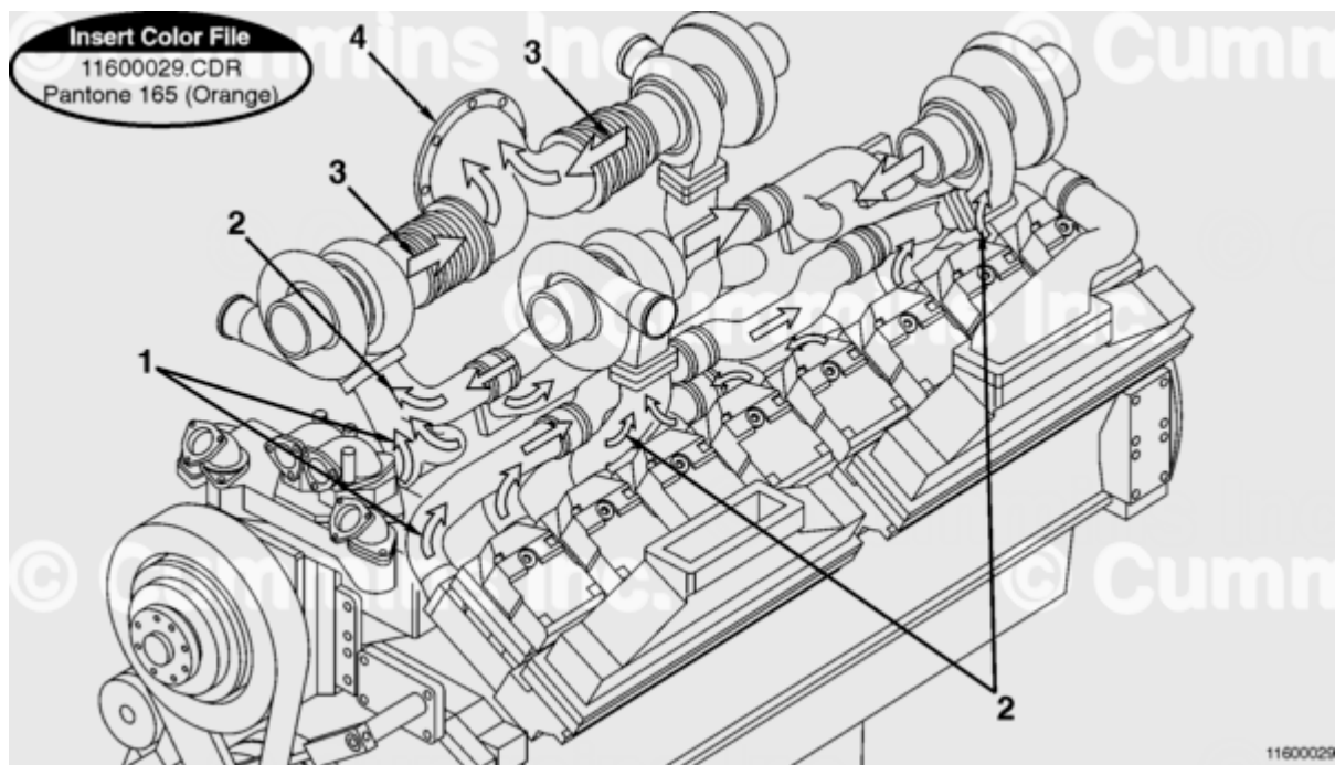
QSK60 Exhaust System - Single-Stage Turbocharger, Aftercooled
