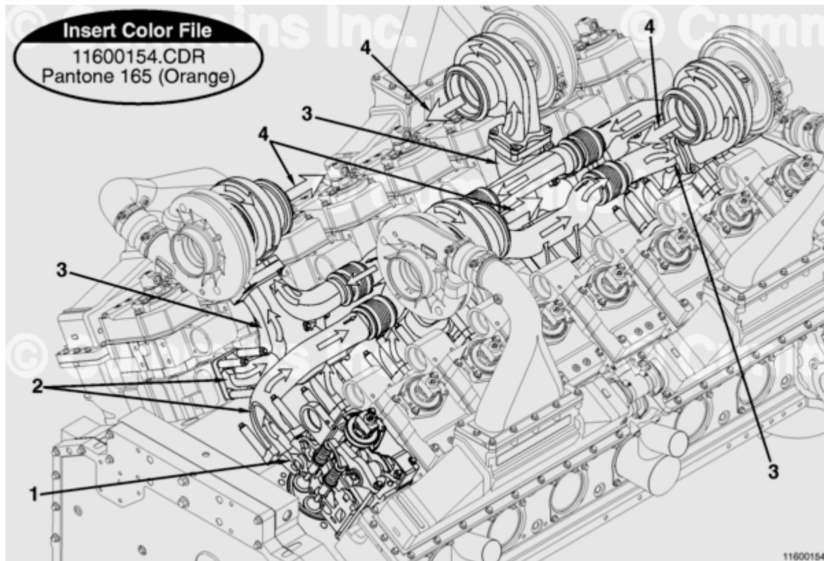
QSK60 Exhaust System - Single-Stage Turbocharger, Aftercooled
