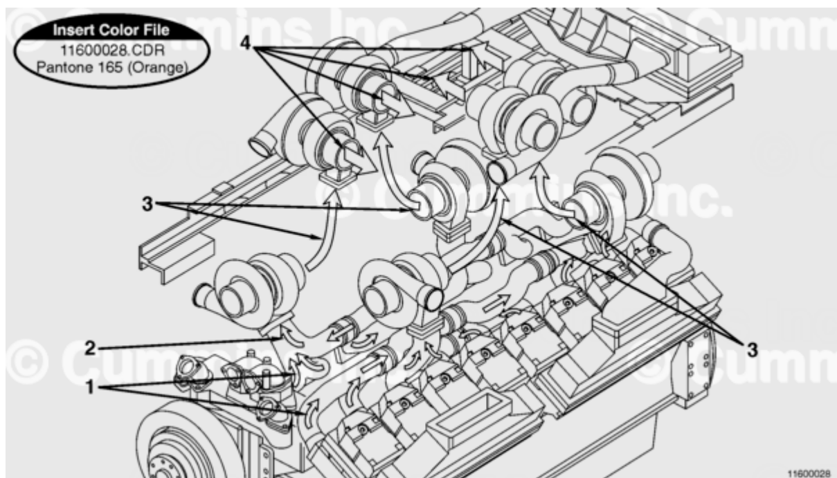
QSK60 Exhaust System - Two-Stage Turbocharger, Aftercooled and Intercooled
