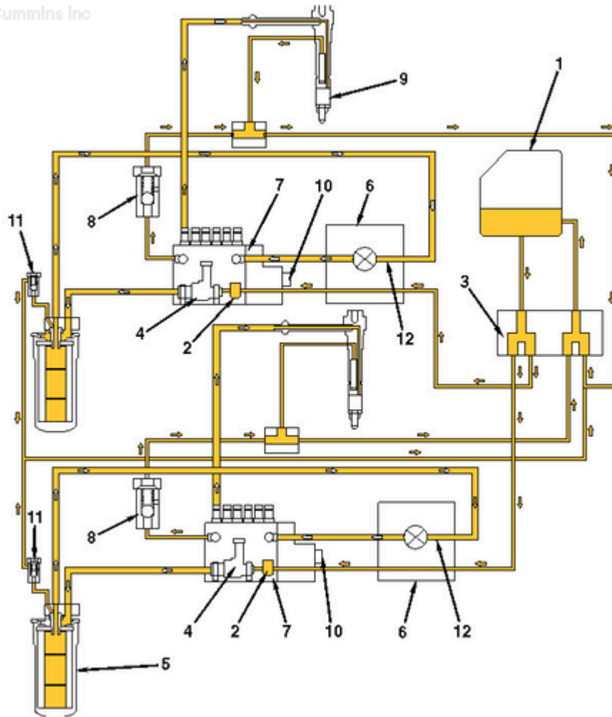
Generator-Drive Fuel System with Mechanical Lift Pumps
