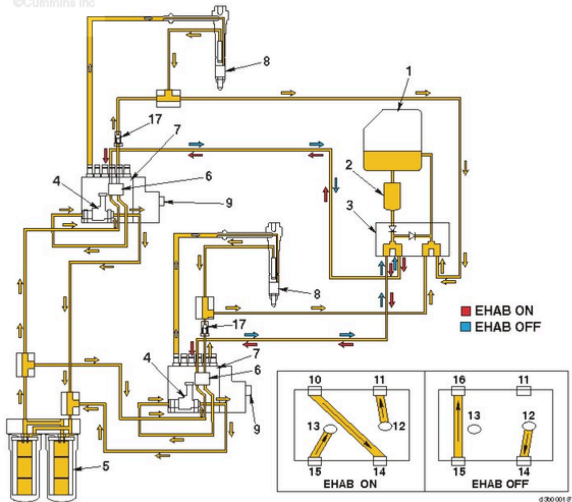
Industrial Fuel System with EHAB and Mechanical Lift Pumps
