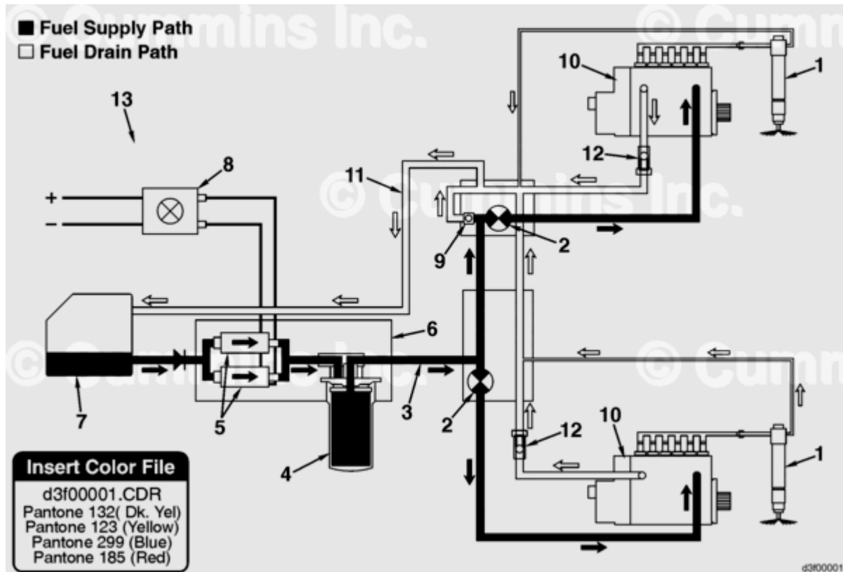
Industrial and Generator-Drive Fuel System with Electric Lift Pumps
