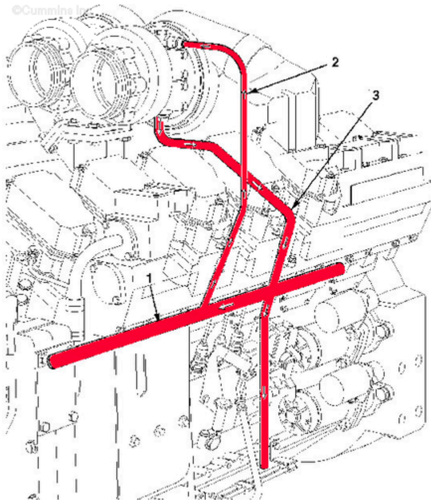
Turbocharger
