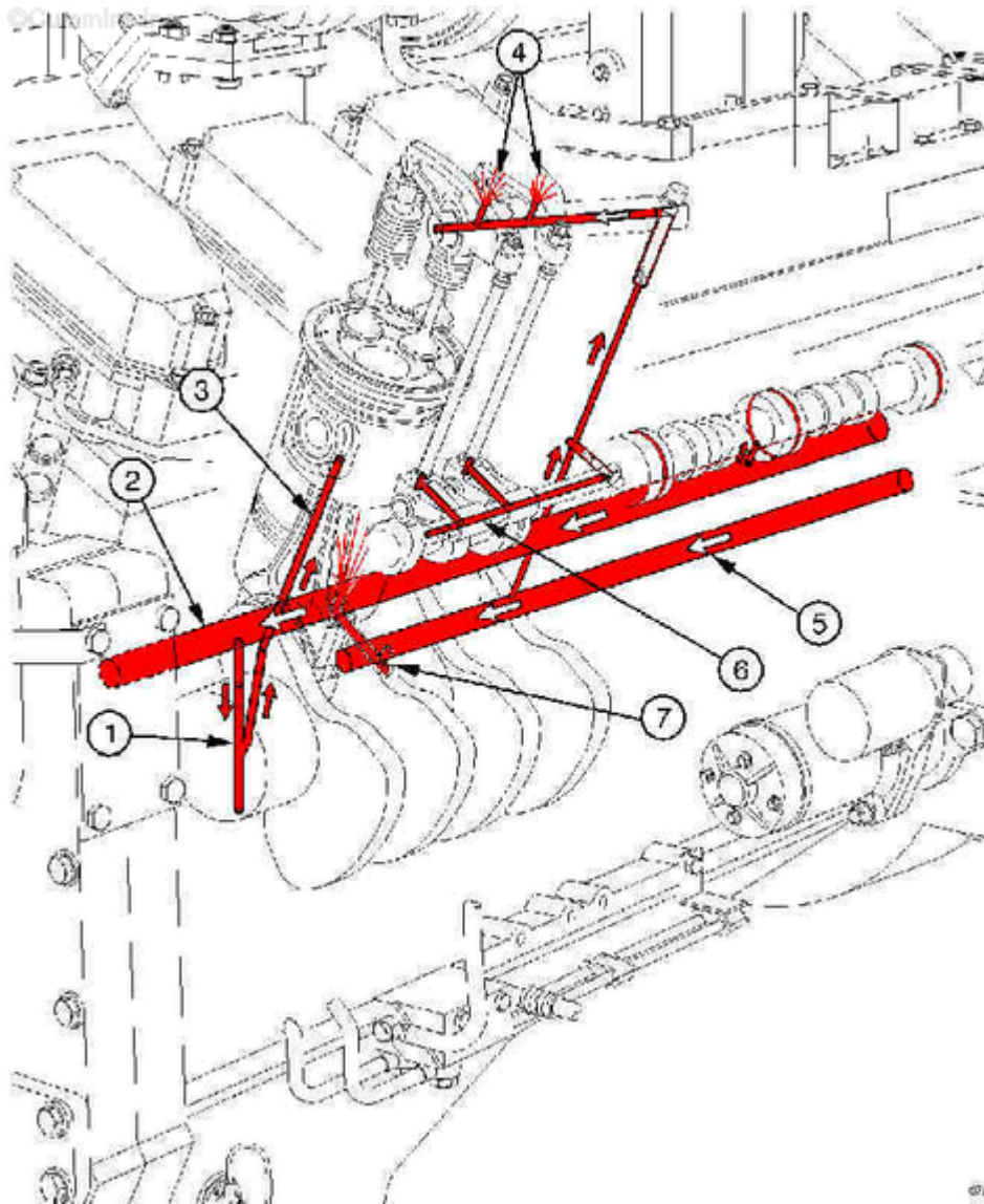
Piston Cooling, Connecting Rod, Overhead
