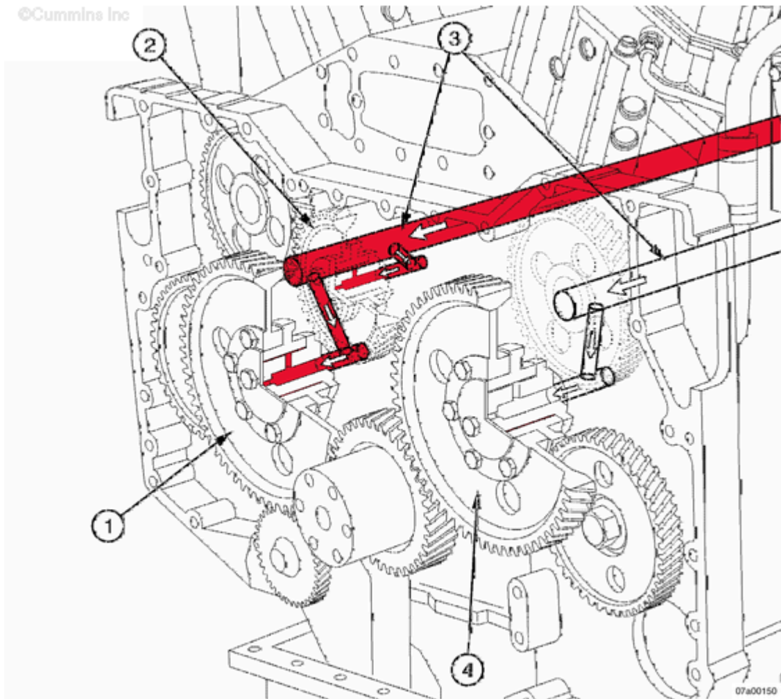
Front Gear Train
