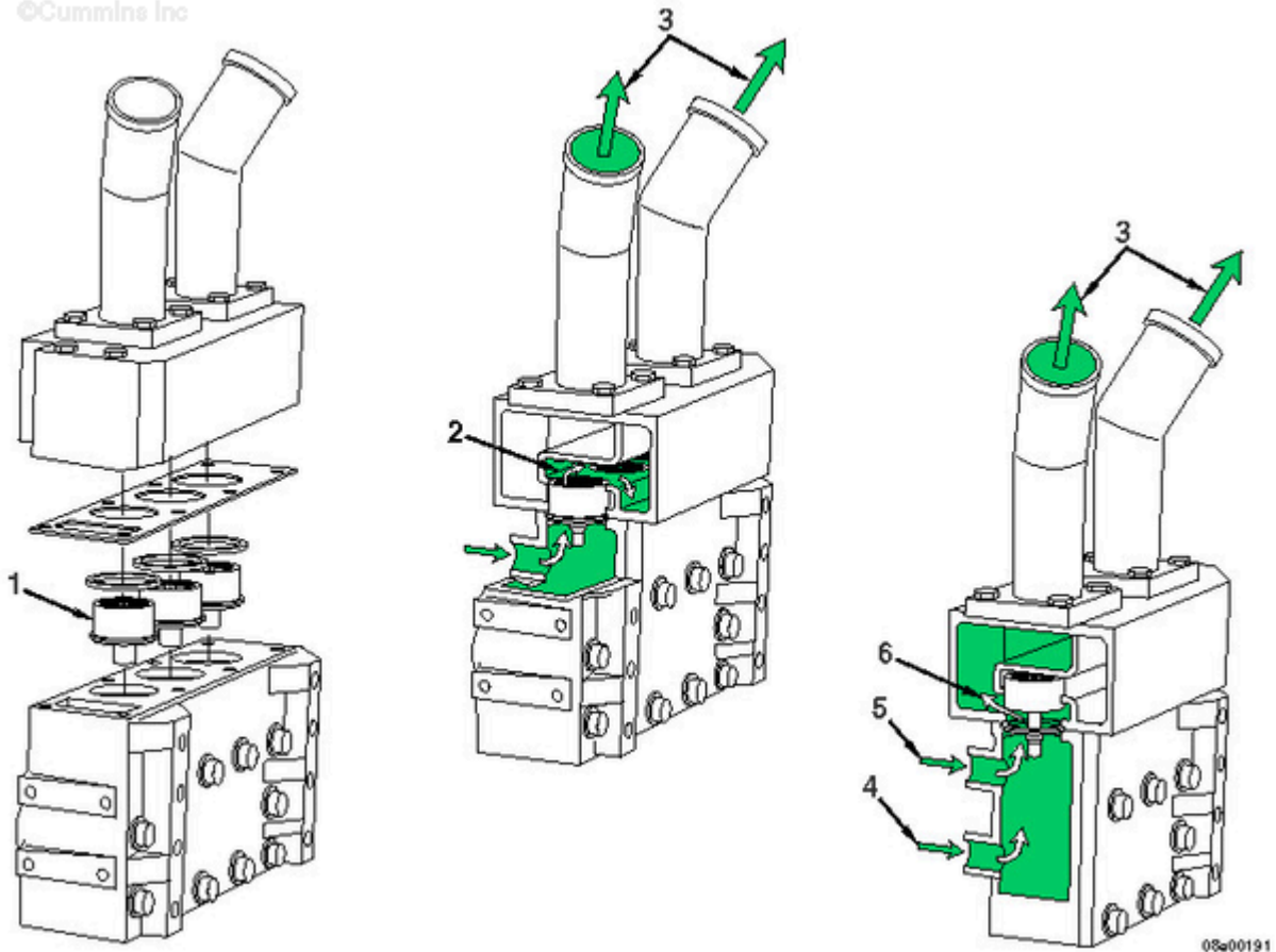
Thermostat Housing Flow
