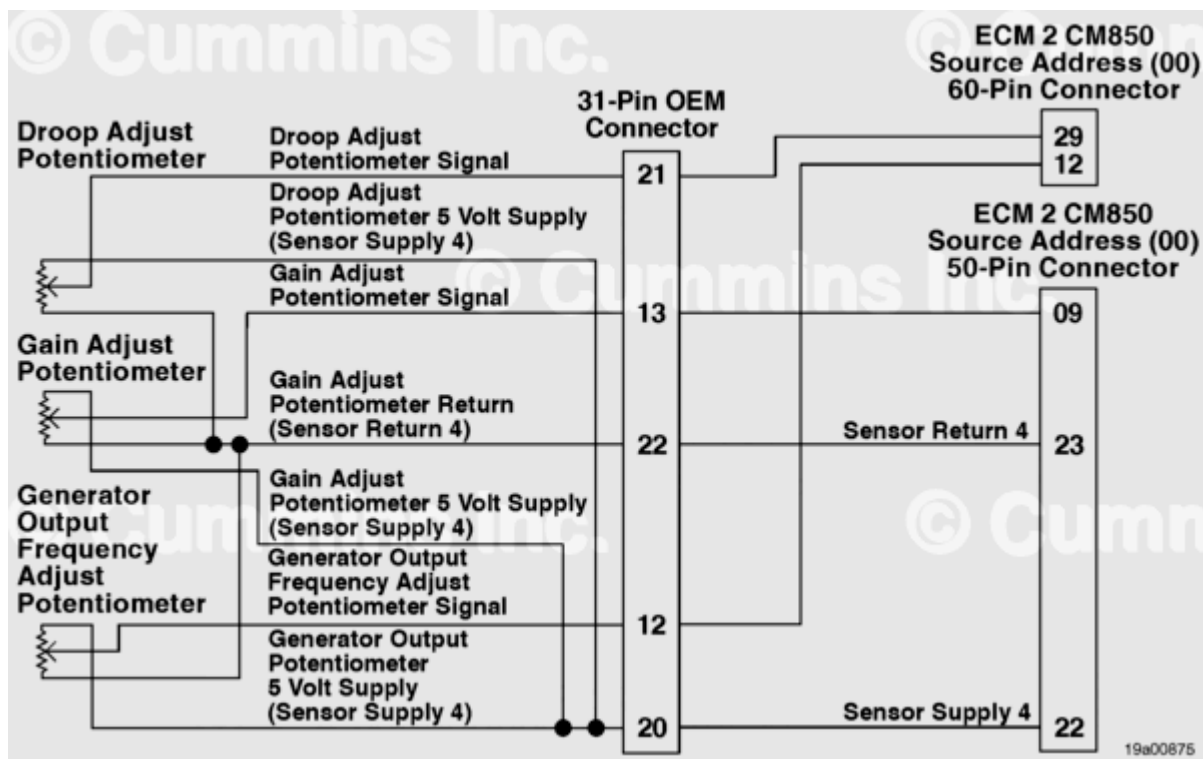
Droop Adjust Potentiometer Circuit
