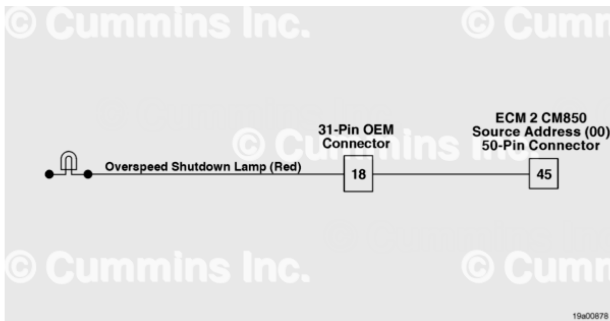
Overspeed shutdown lamp Circuit
