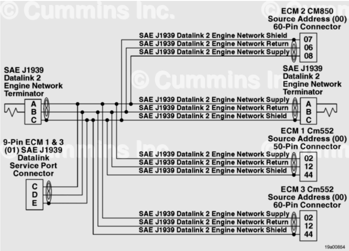
Engine Control Module (ECM)
