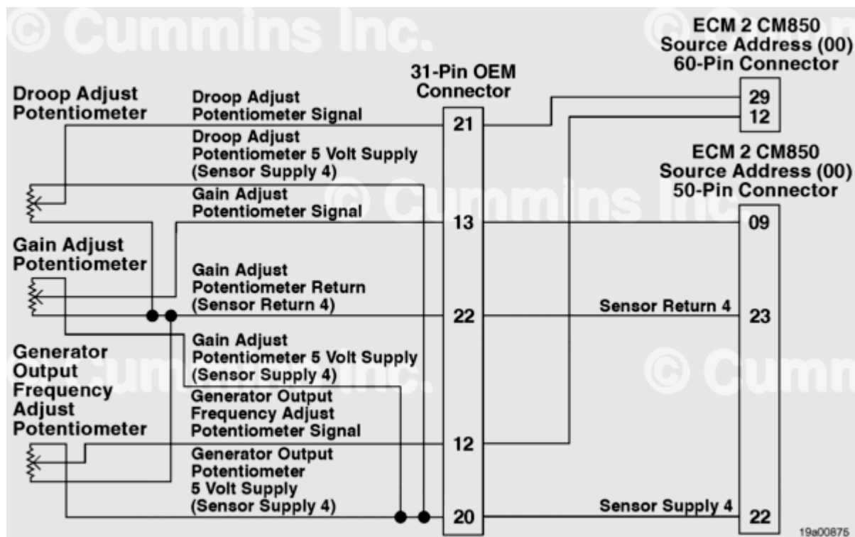
Sensor Supply 4 Circuit
