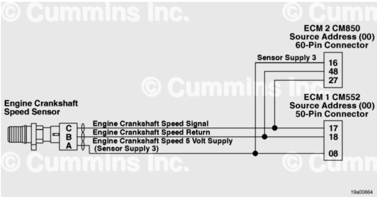
Sensor Supply 3 Circuit
