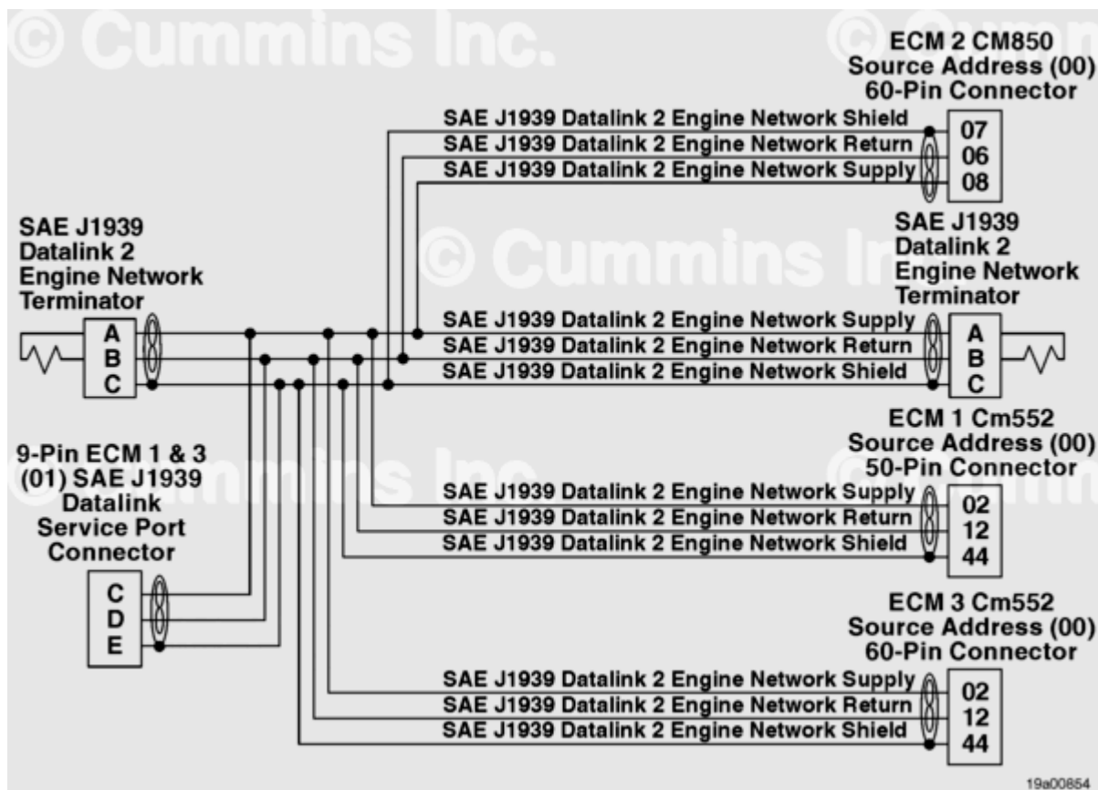
J1939 Data Link 2 Engine Network Circuit
