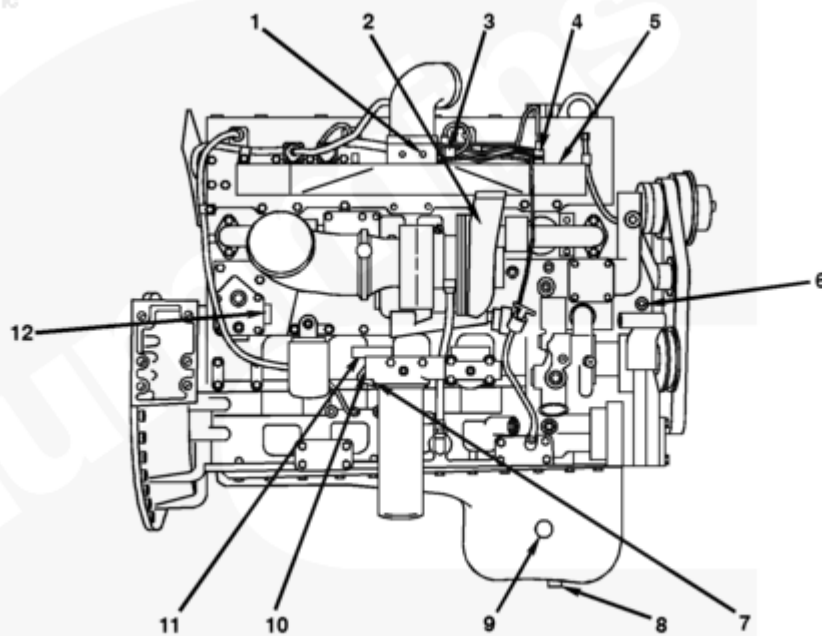
Exhaust Side
