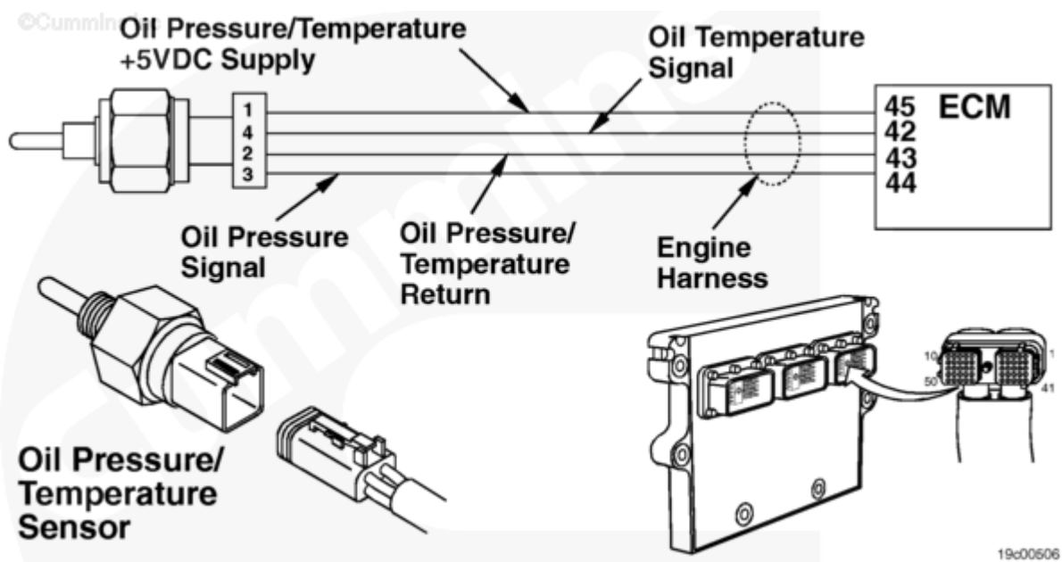
Oil Pressure Sensor Circuit
