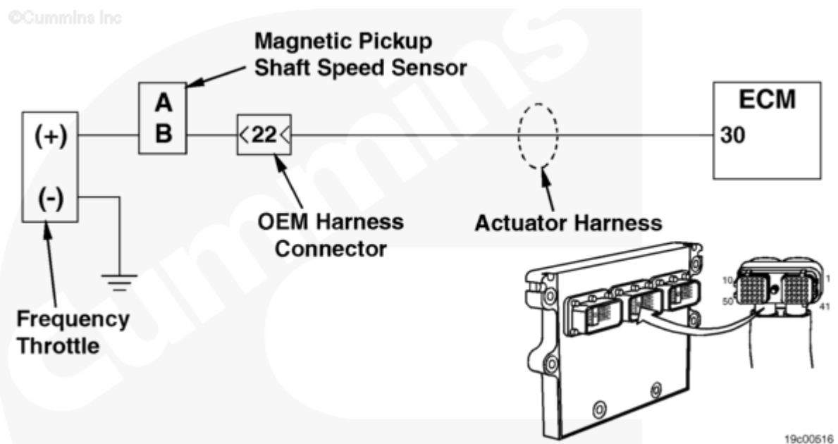
Frequency Throttle Circuit
