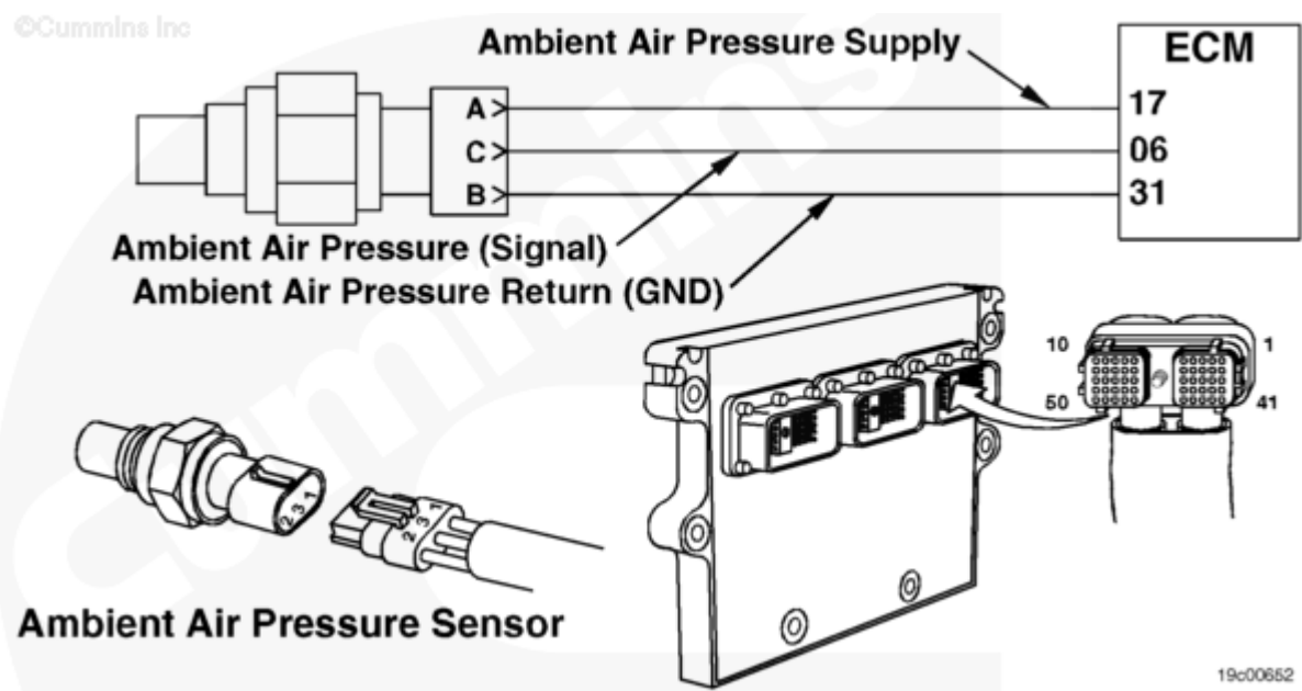
Ambient Air Pressure Sensor Circuit
