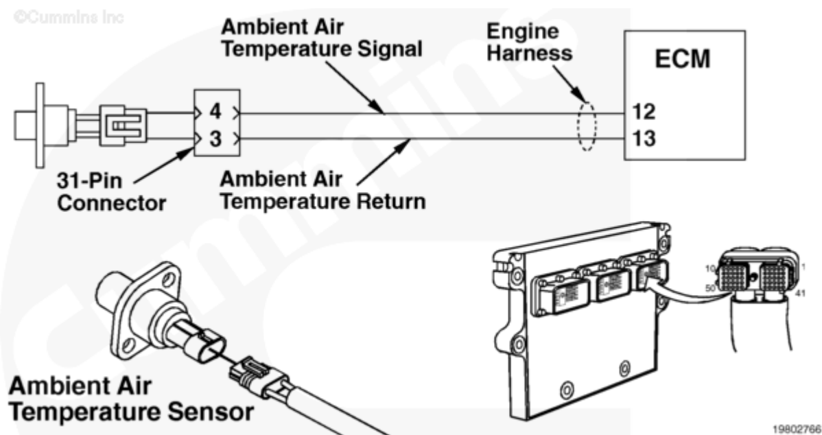
Ambient Air Temperature Sensor Circuit
