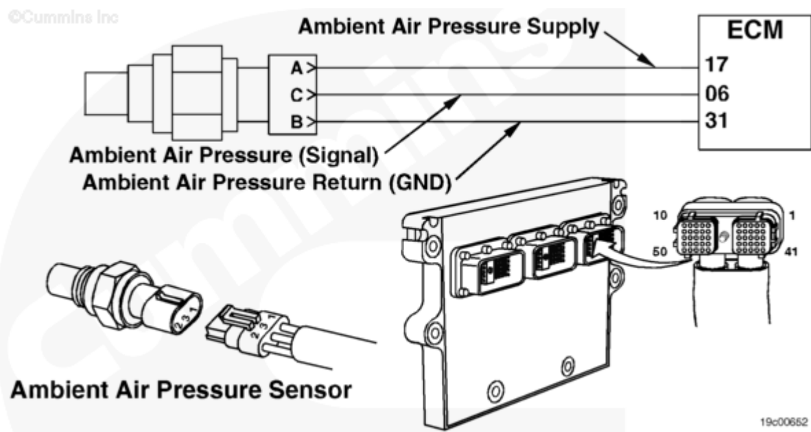
Ambient Air Pressure Sensor
