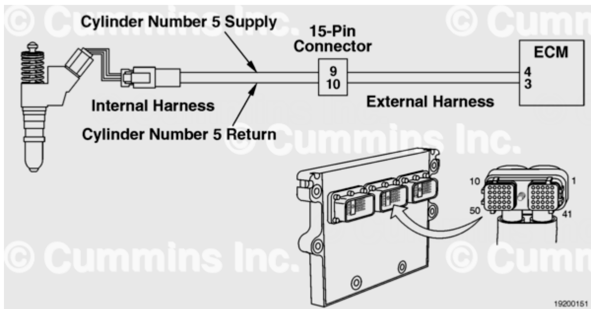
Injector Circuit
