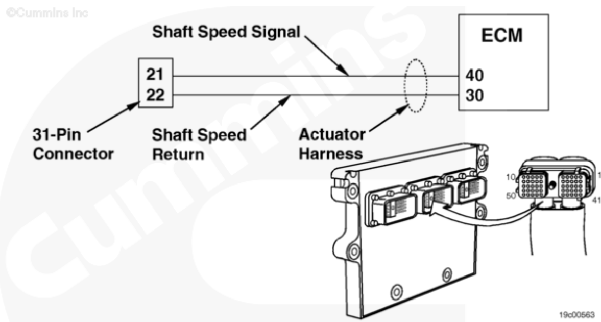
Auxiliary Speed Governor Circuit
