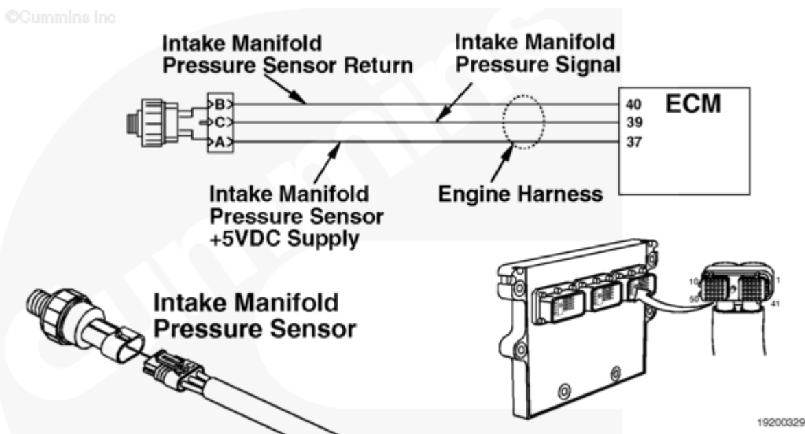
Intake Manifold Pressure Sensor
