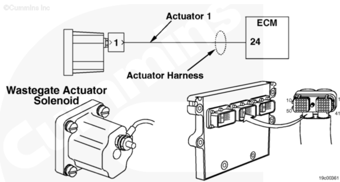
Wastegate Actuator number 1 Circuit
